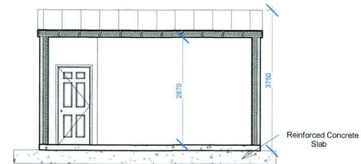
Section View
