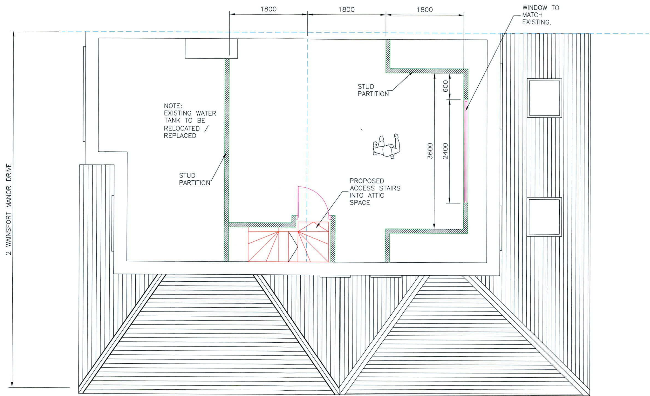
PROPOSED ATTIC FLOOR PLAN VIEW
