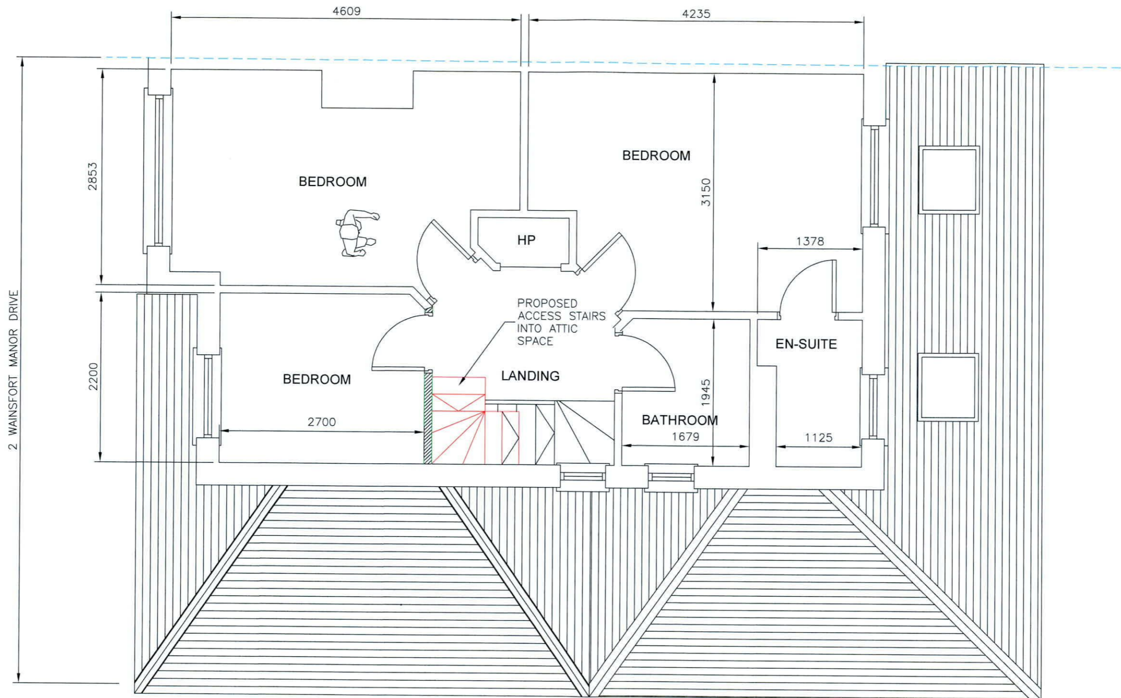
PROPOSED FIRST FLOOR PLAN VIEW
