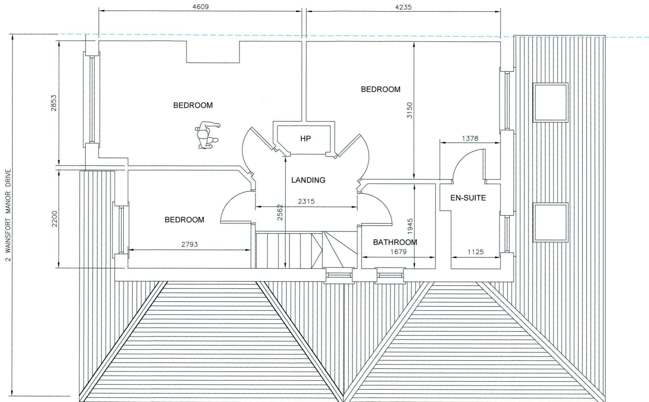
EXISTING FIRST FLOOR PLAN VIEW
