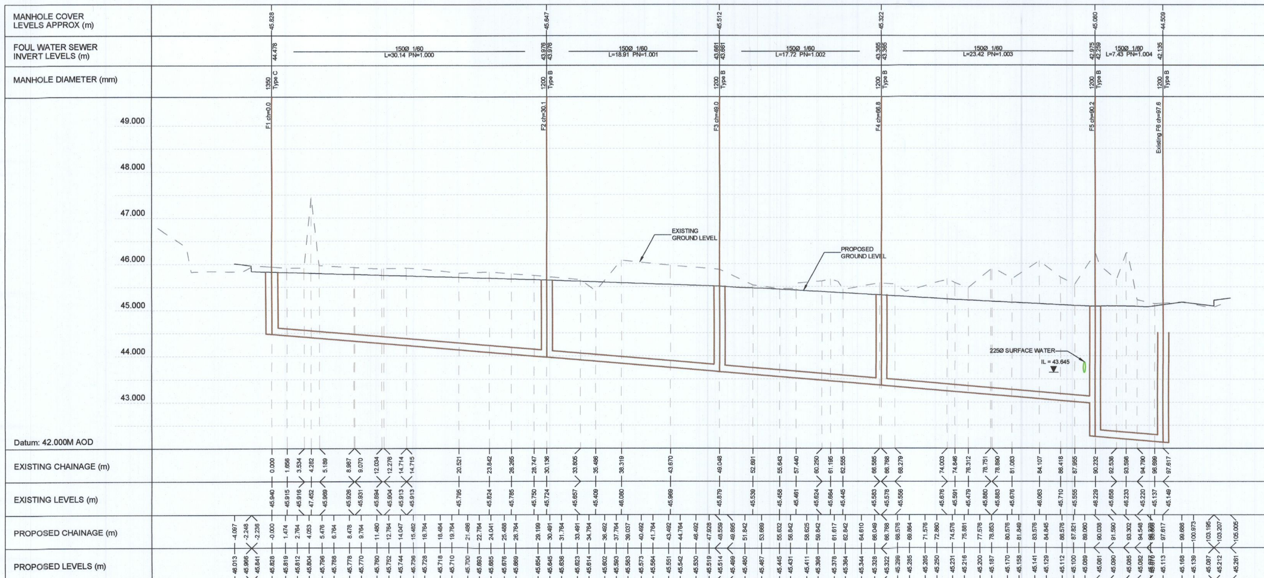
PROPOSED FOUL SEWER LONGITUDINAL SECTION
