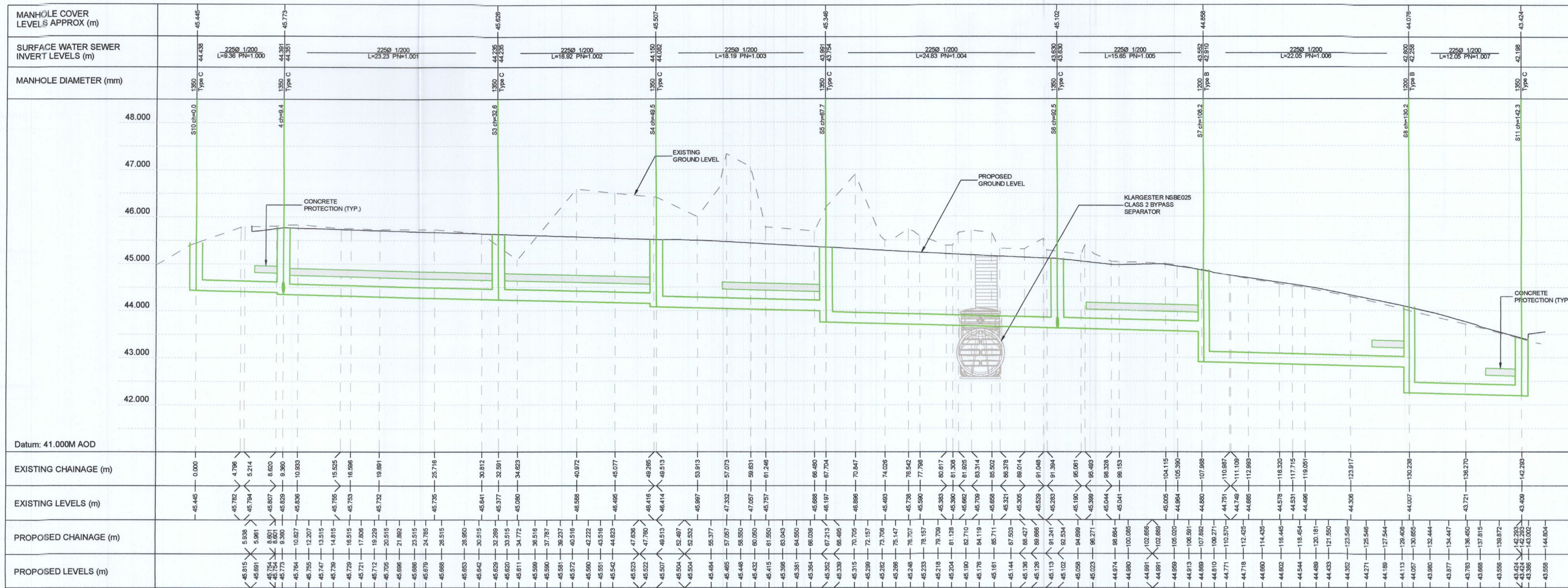
PROPOSED SURFACE WATER LONGITUDINAL SECTION
