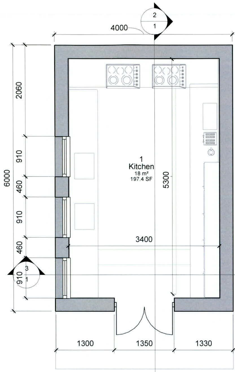
1 Ground Floor 1:50
