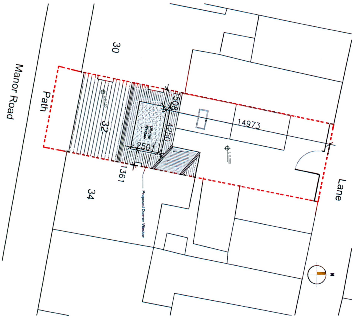
Site Plan
