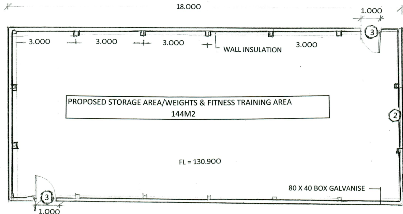
PLAN SCALE 1:100
