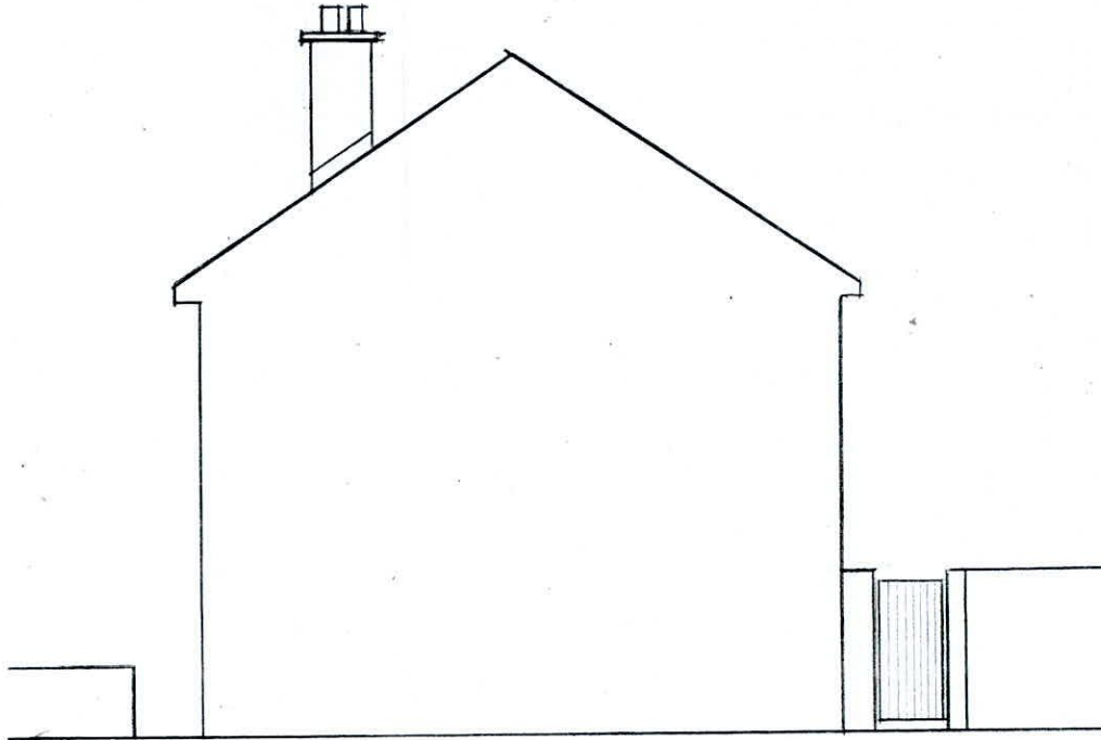
Existing Side Elevation [from no.106.] scale 1:100.
