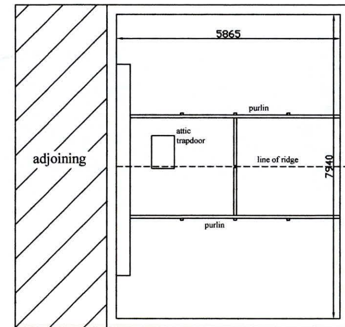
ROOF SPACE FLOOR PLAN
