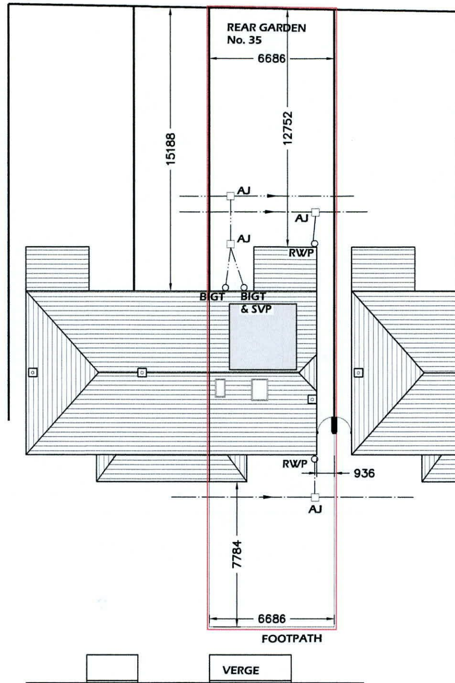
Proposed Block Plan & Drainage Layout SCALE 1:200
