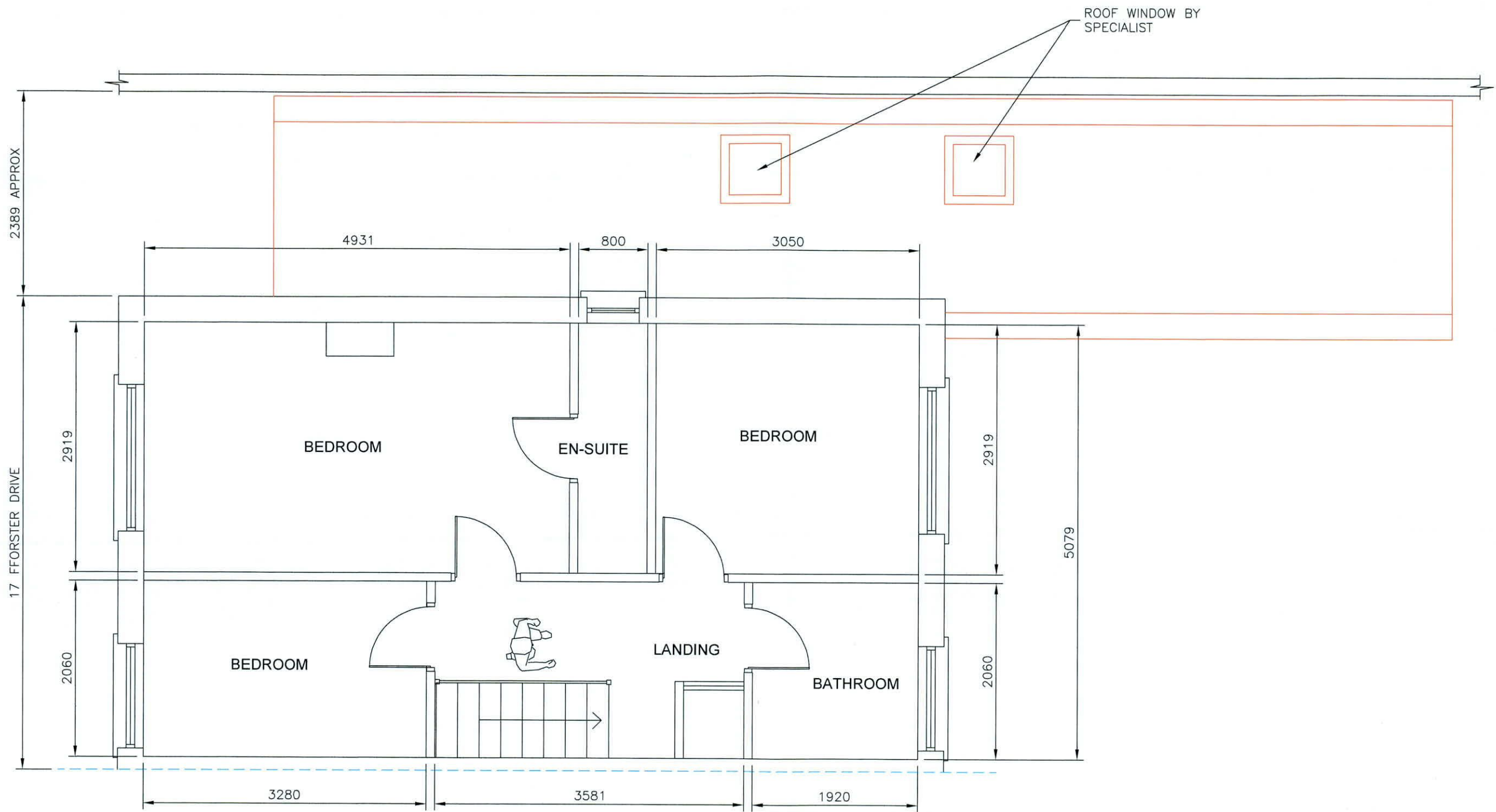
PROPOSED FIRST FLOOR PLAN VIEW
