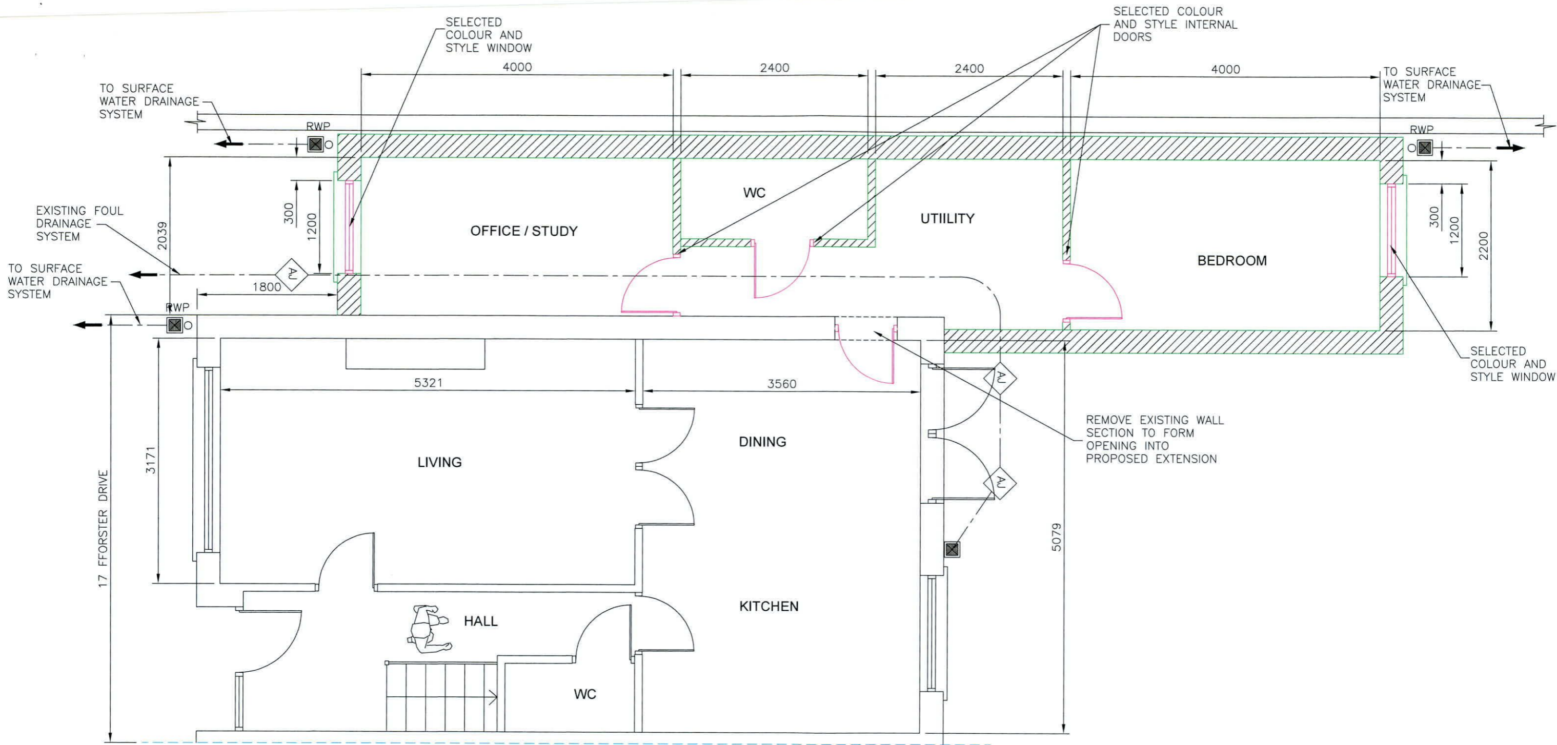
PROPOSED GROUND FLOOR PLAN VIEW
