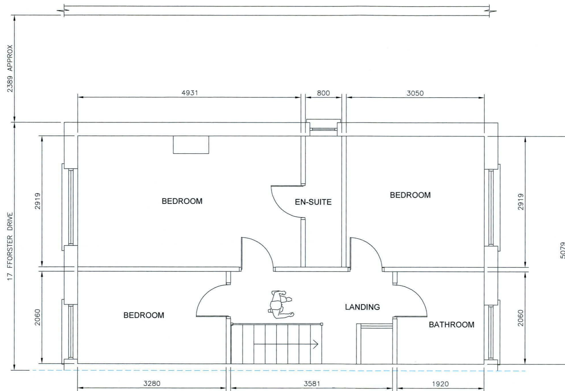
EXISTING FIRST FLOOR PLAN VIEW
