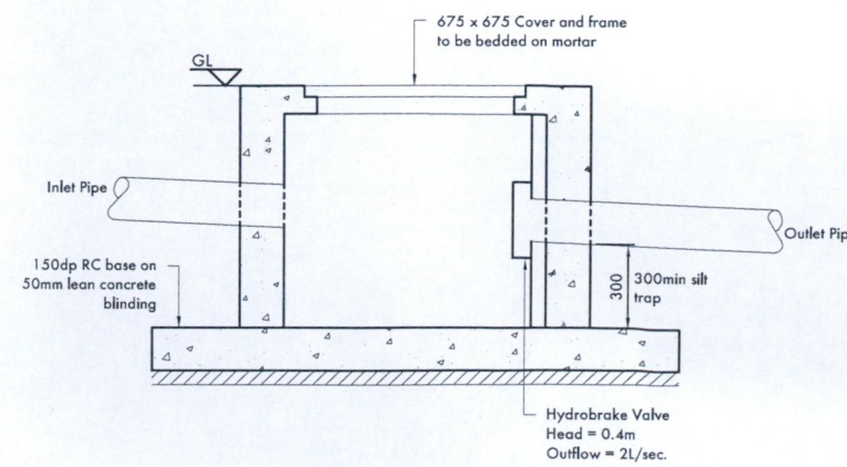
DETAIL SWMH Scale 1:20
