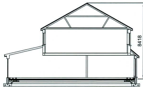
TYPICAL SECTION
