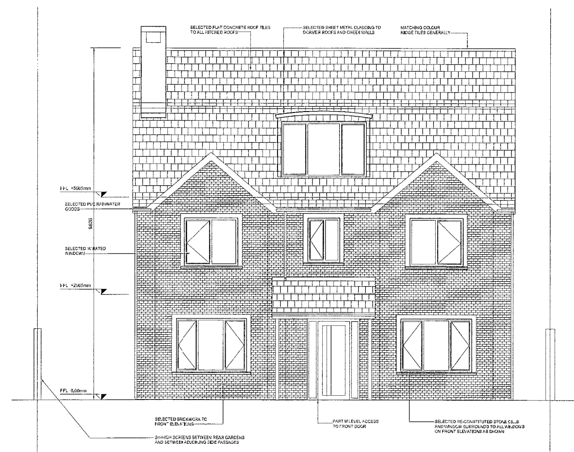
FRONT ELEVATION
