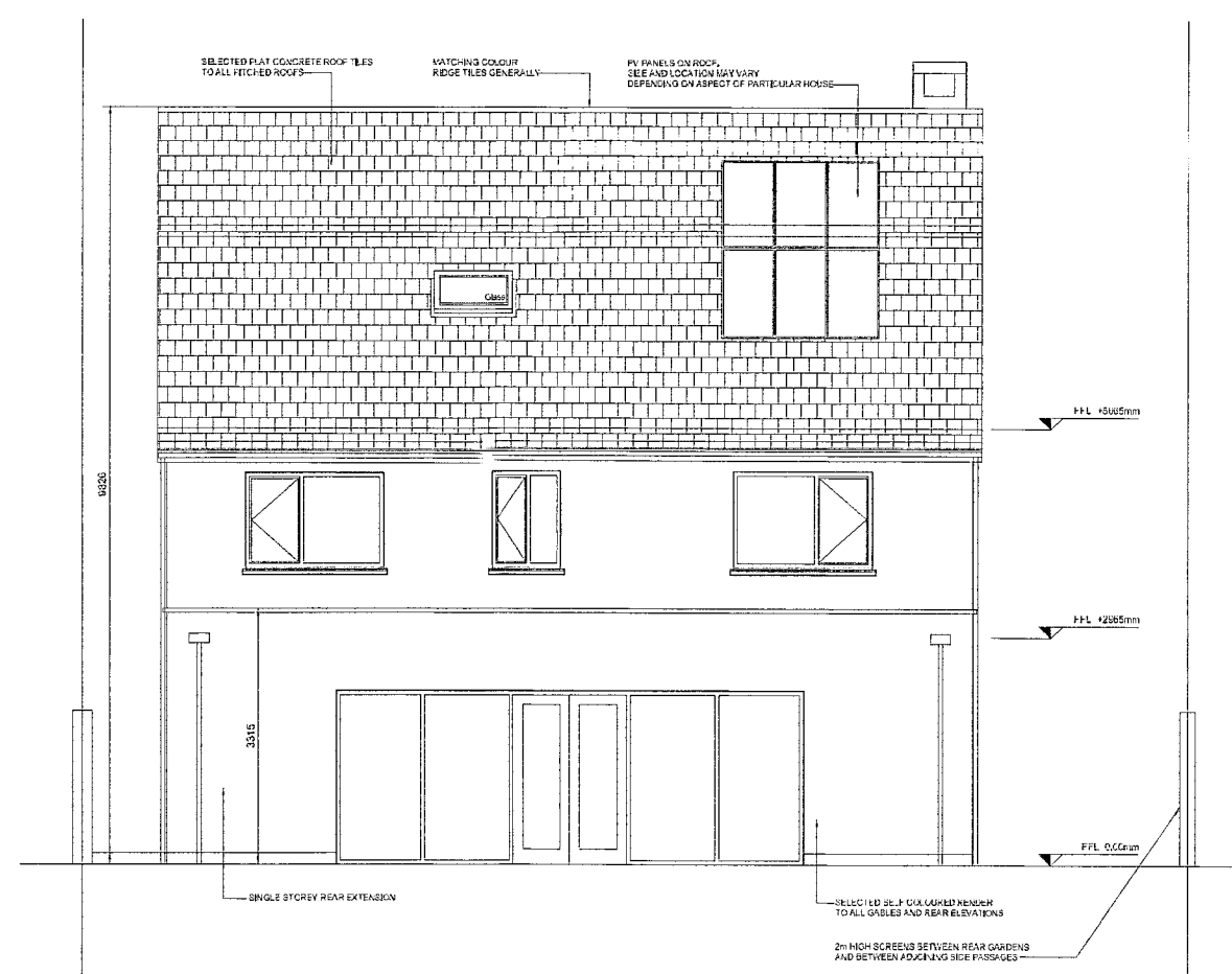
REAR ELEVATION
