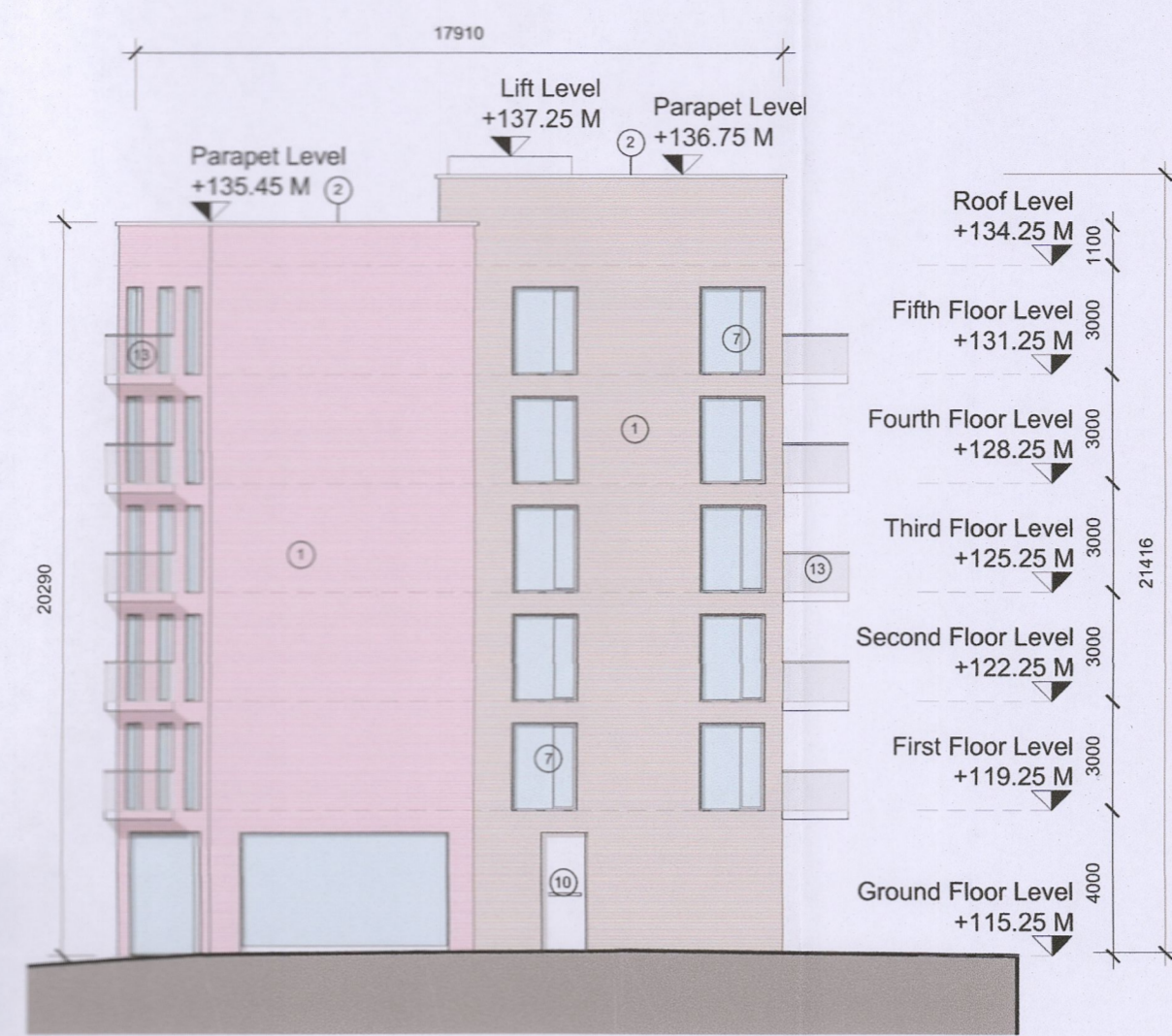
1 PERMITTED - BLOCK E - SOUTH ELEVATION - PLANNING REF ABP-305556-19 Scale: 1 : 200
