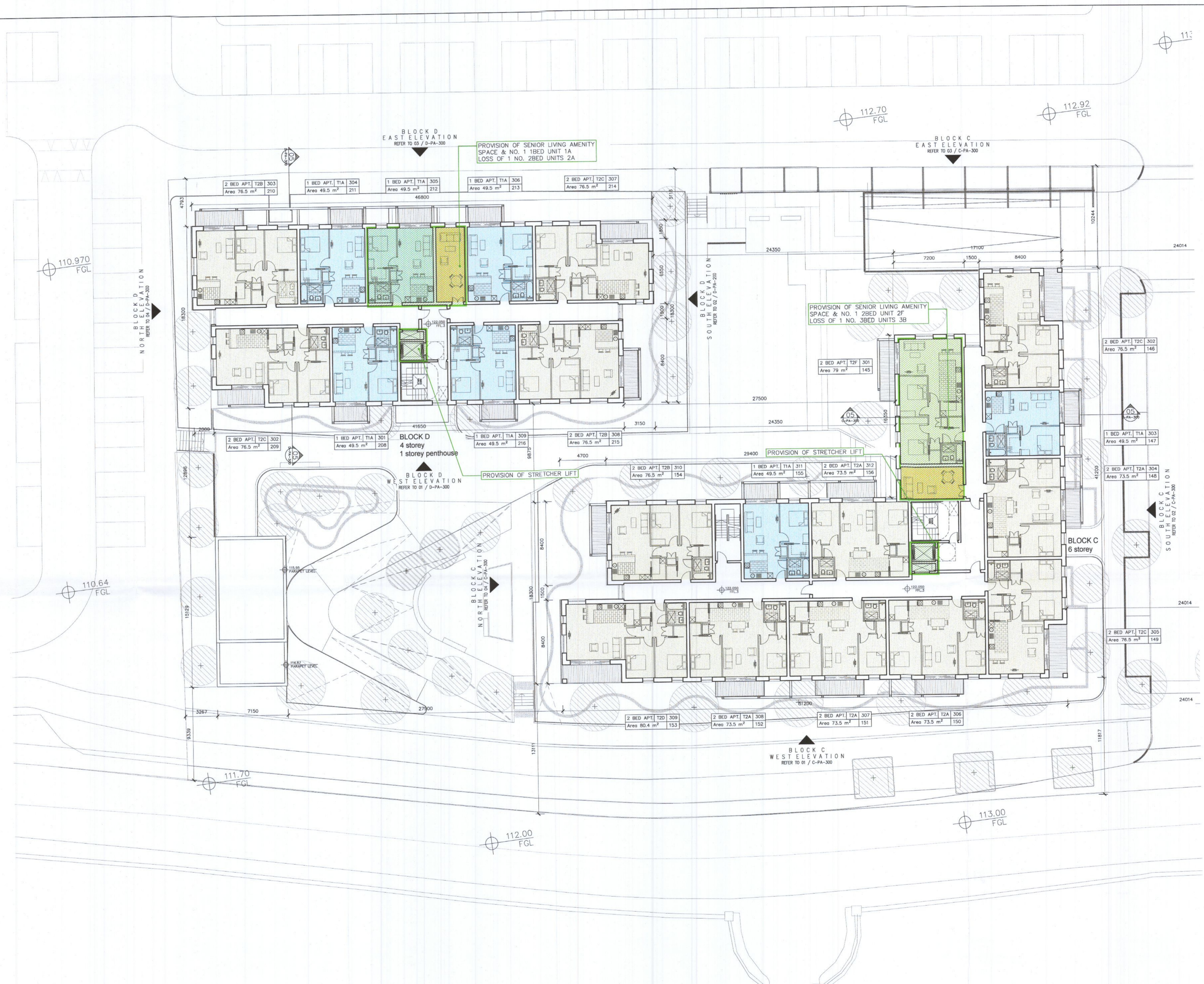
01 Proposed Third Floor Plan PA 104 CD 1:200
