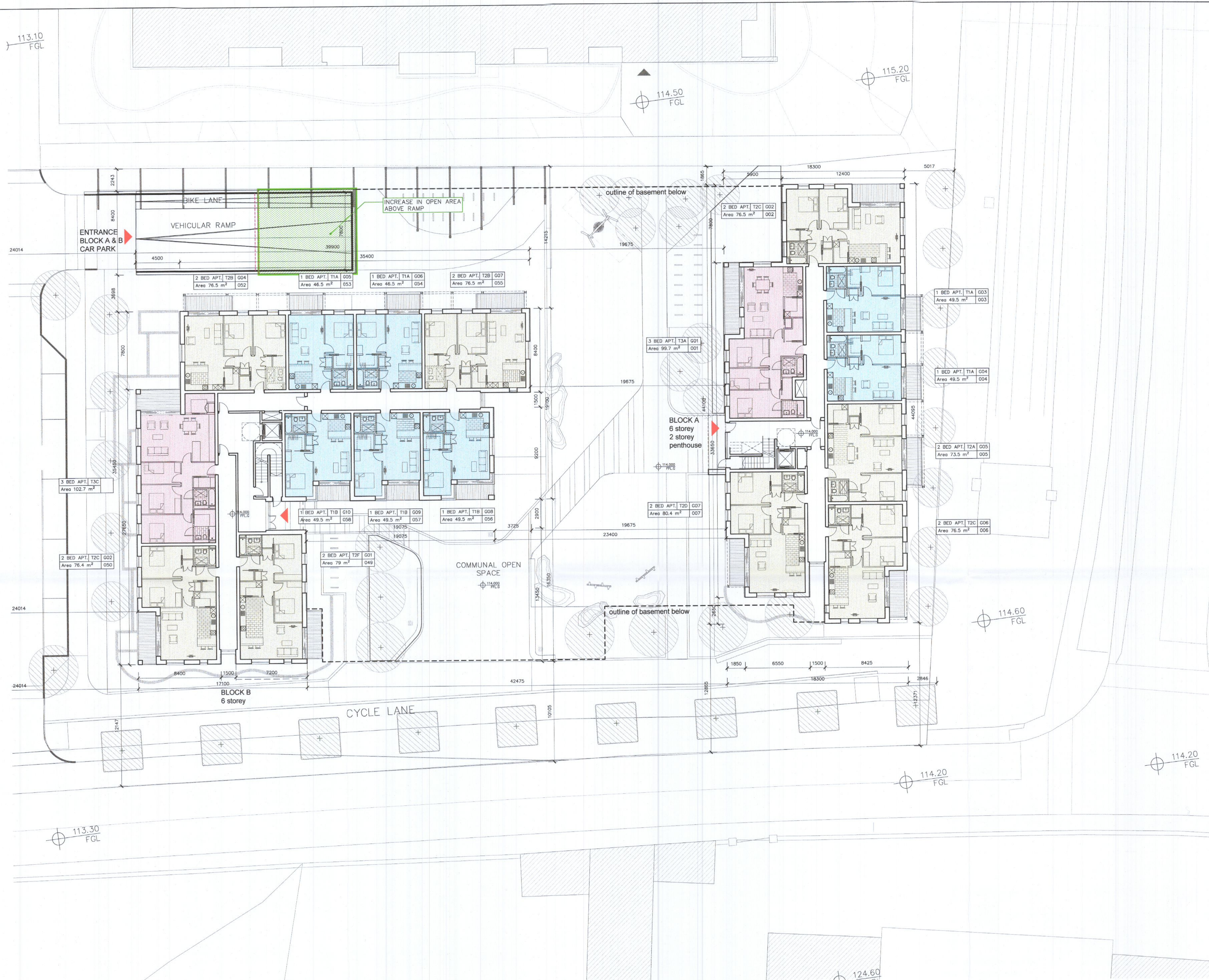
01 Proposed Ground Floor Plan PA 101 AB 1:200
