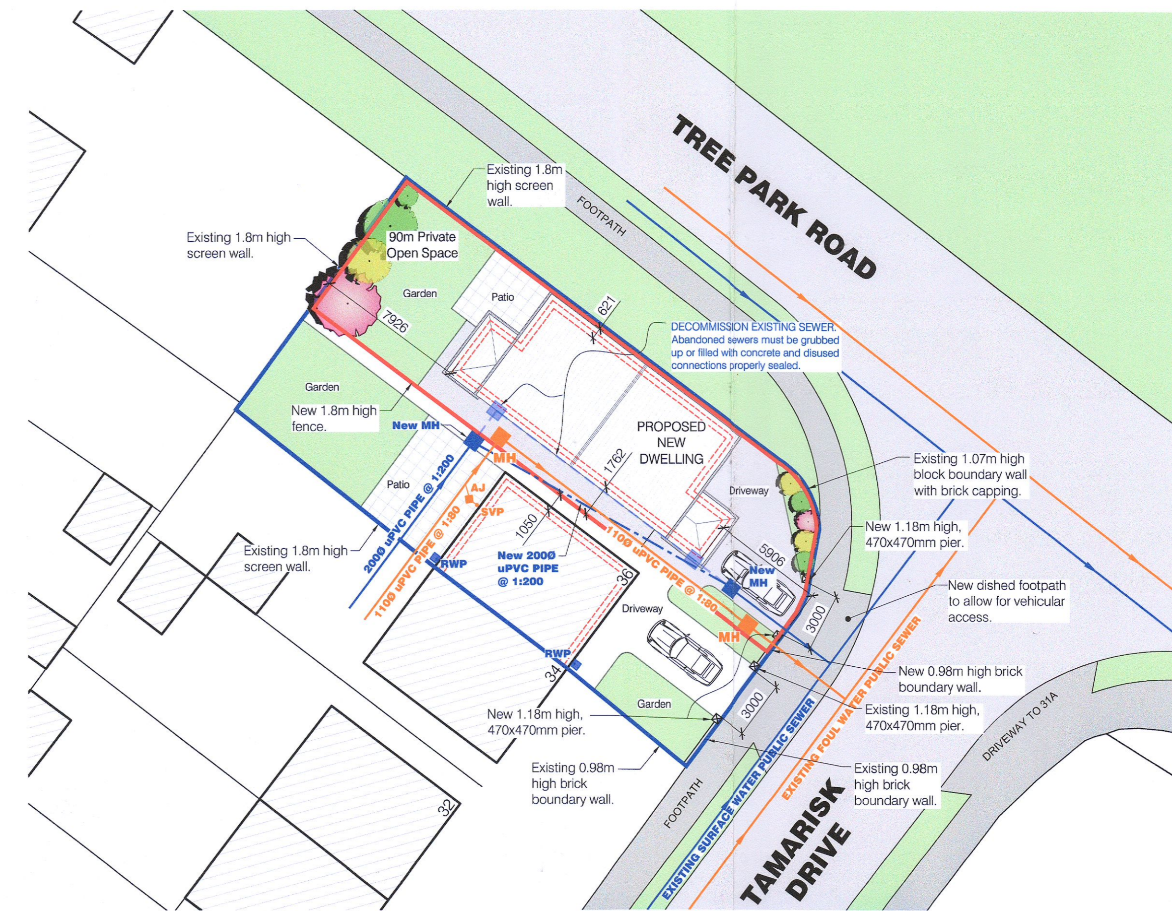
PROPOSED SITE LAYOUT PLAN
