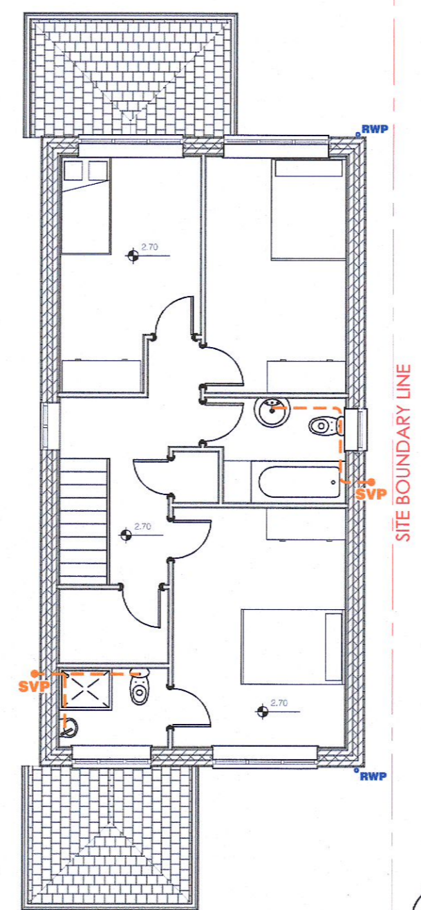
PROPOSED FIRST FLOOR DRAINAGE LAYOUT
