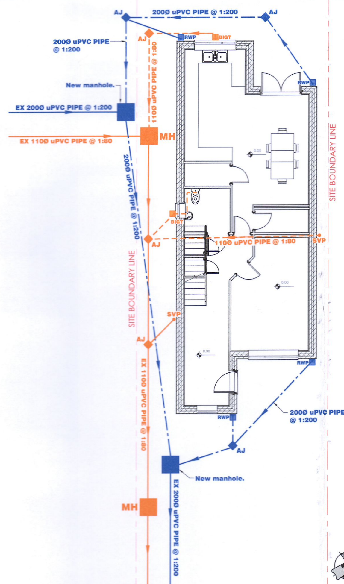
PROPOSED GROUND FLOOR DRAINAGE LAYOUT
