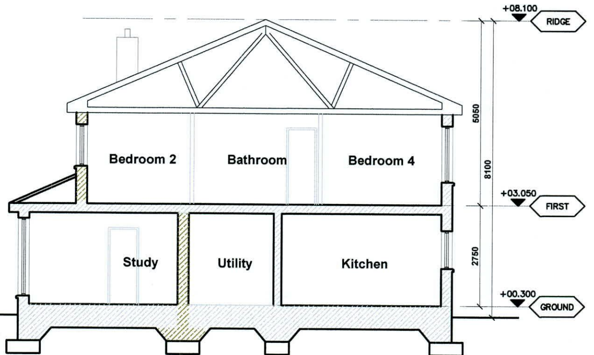
Existing Section B-B Scale - 1:100
