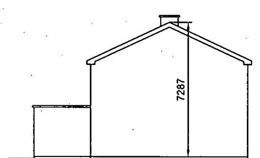
SIDE ELEVATION
