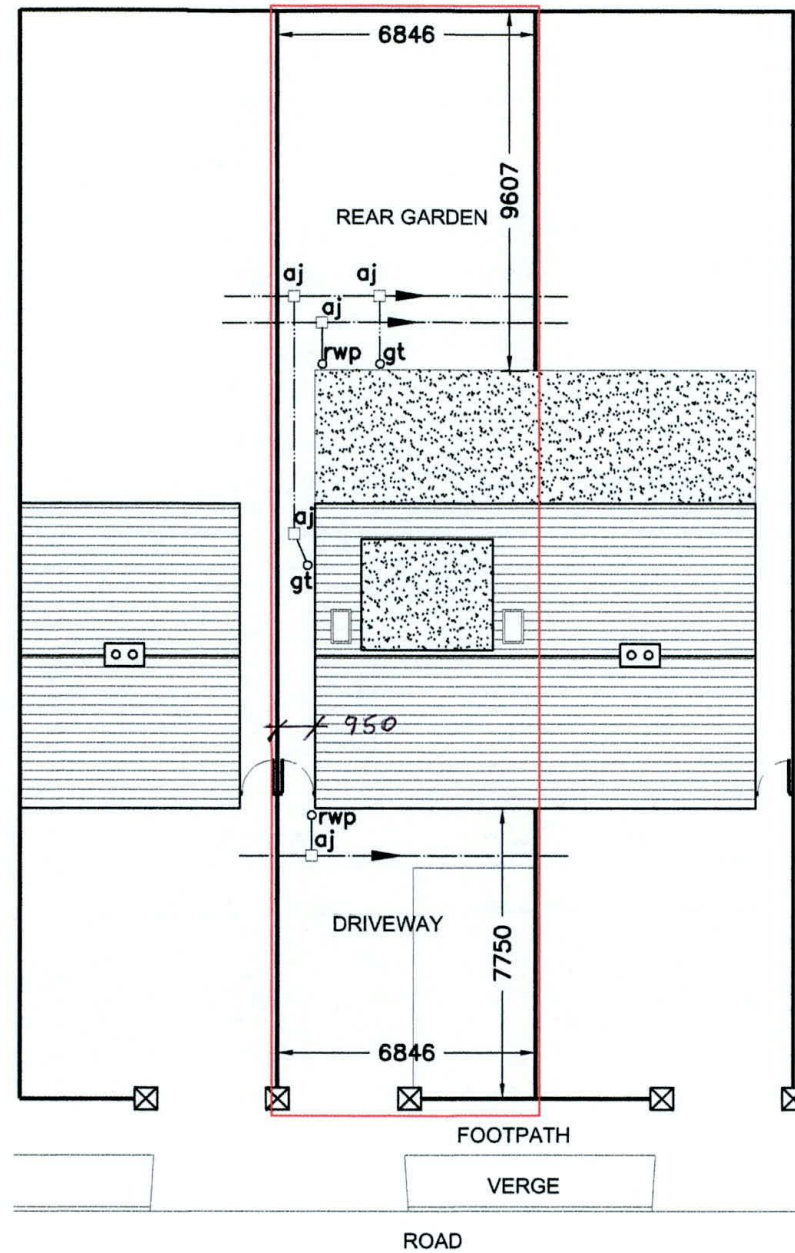
⊕ Proposed Block Plan & Drainage Layout SCALE 1:200
