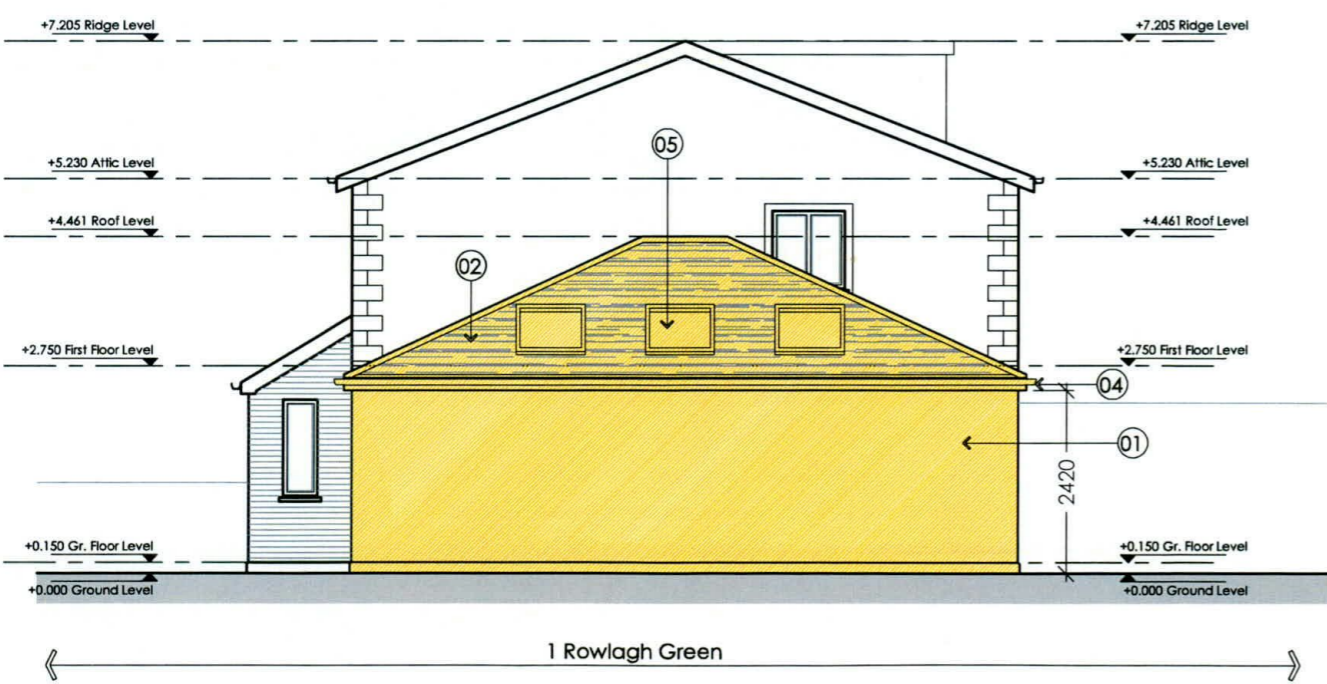
005 Side Gable Elevation - PROPOSED 03 1:100
