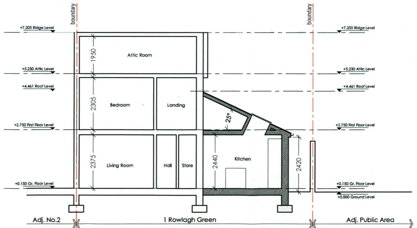
005 Section A-A - PROPOSED 04 1:100
