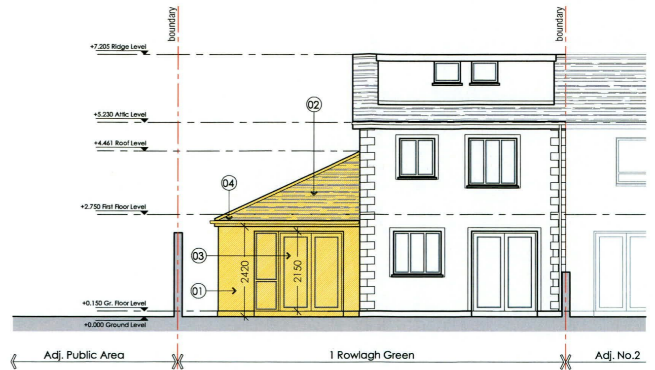
005 Rear Elevation - PROPOSED 02 1:100
