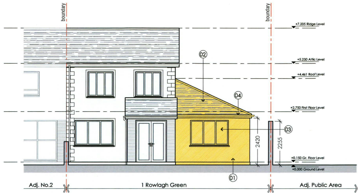
005 Front Elevation - PROPOSED 01 1:100
