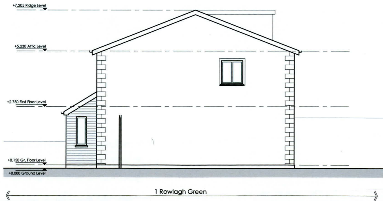
003 Side Gable Elevation - EXISTING 03 1:100
