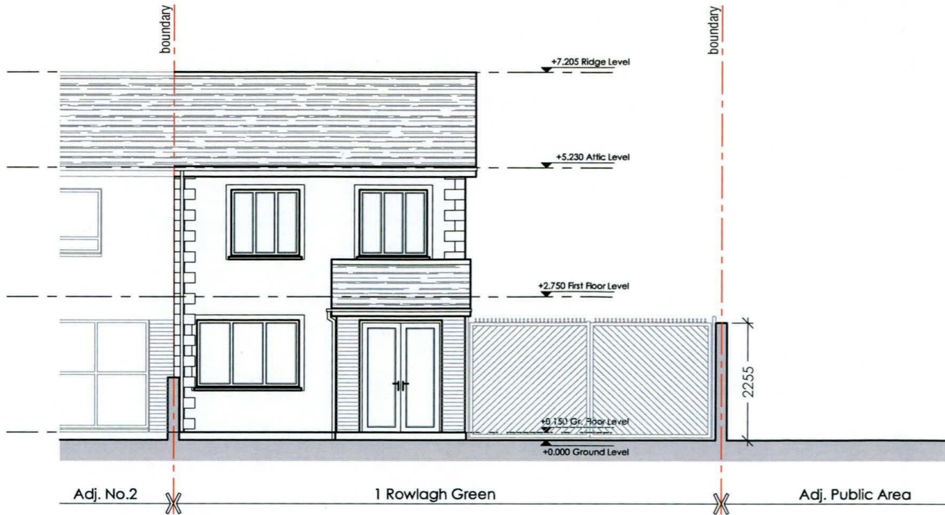
003 Front Elevation - EXISTING 01 1:100
