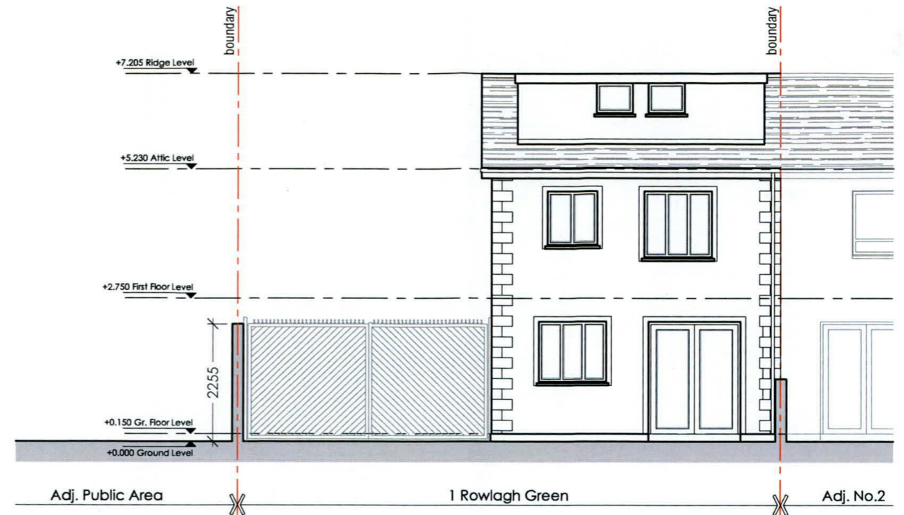
003 Rear Elevation - EXISTING 02 1:100
