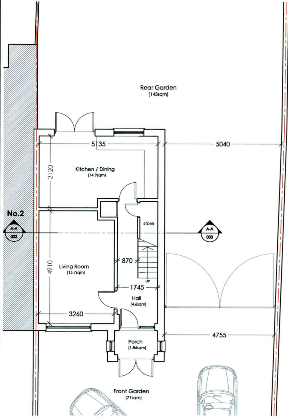
002 Ground Floor Layout Plan - EXISTING 01 1:100
