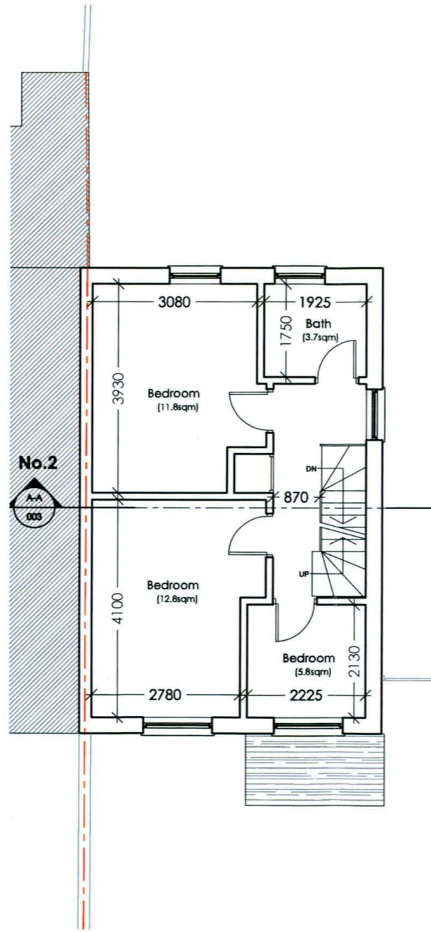
002 First Floor Layout Plan - EXISTING 02 1:100
