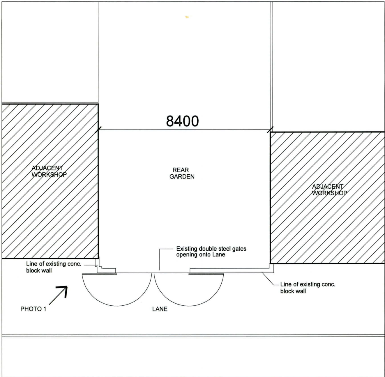
EXISTING LAYOUT PLAN Scale:1:100
