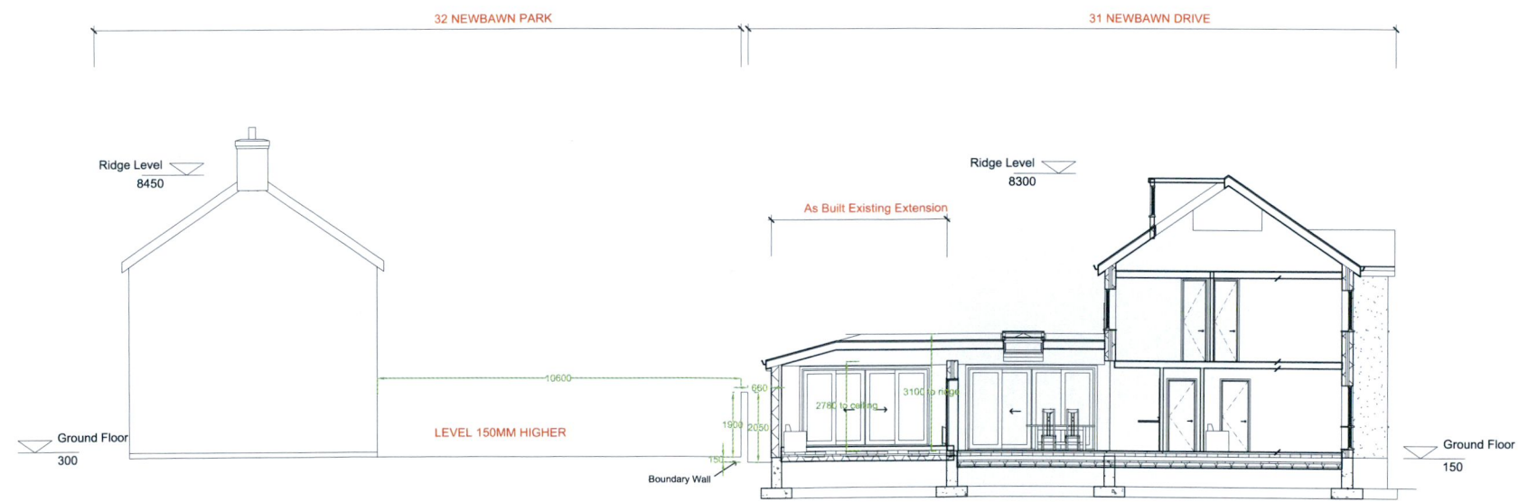
Existing long section + 32 New Bawn Park
