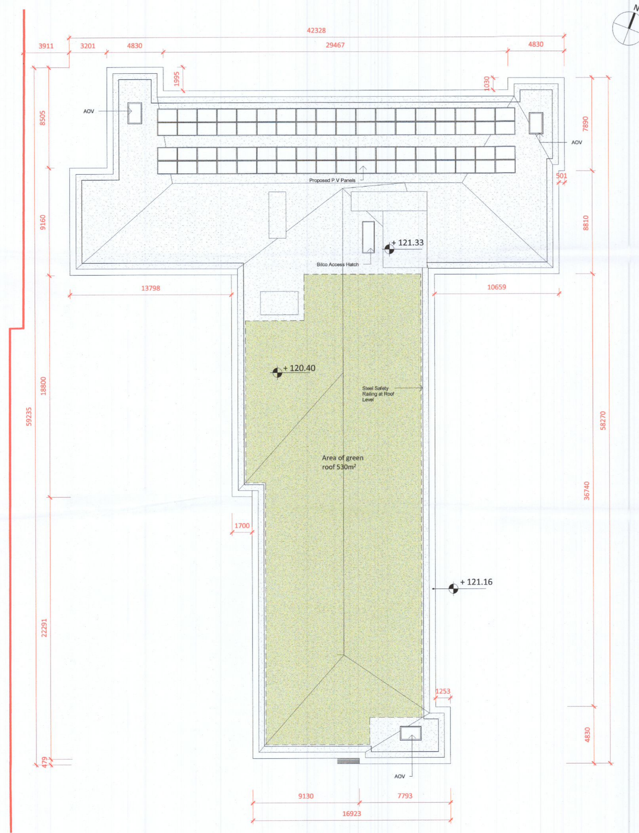
1 05 - Roof Level 1 : 200
