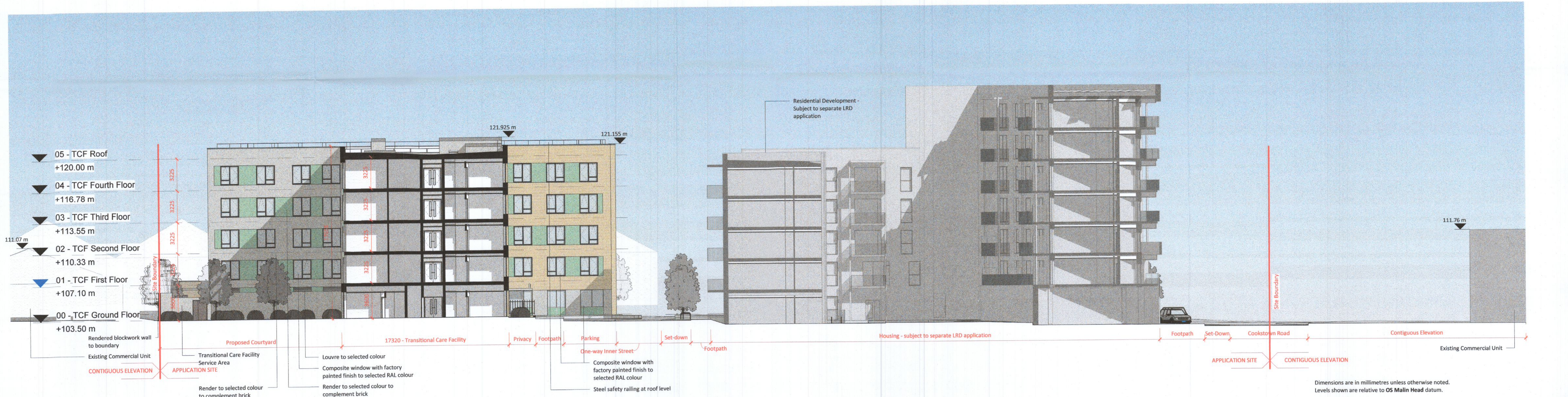
1 Proposed Section A-A - Transitional Care Facility 1:200
