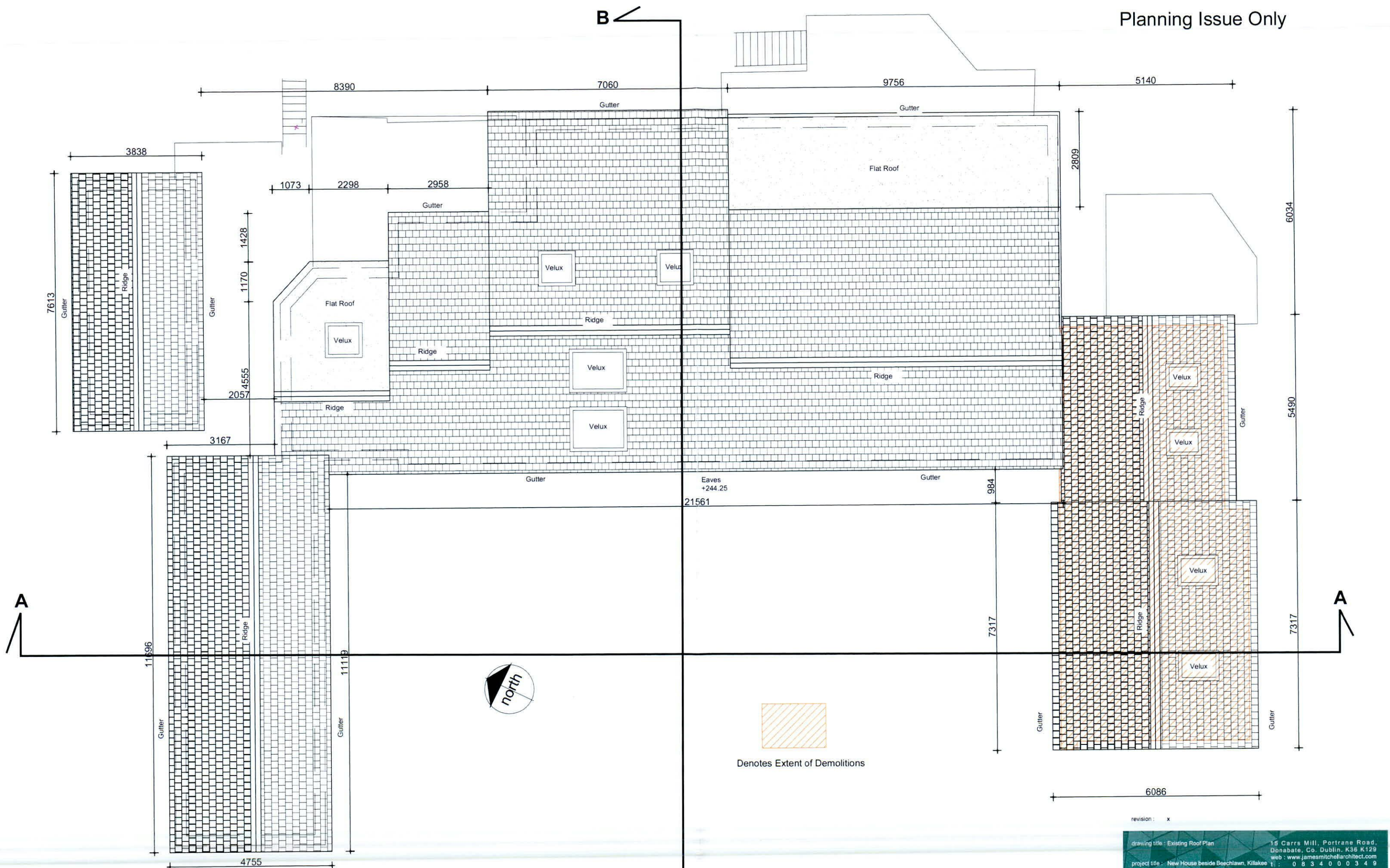
Roof Plan
