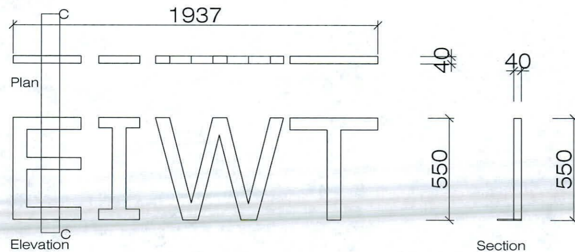
Weston Airport Airport ID Sign Plan/section/elevation 3 111 1:20
