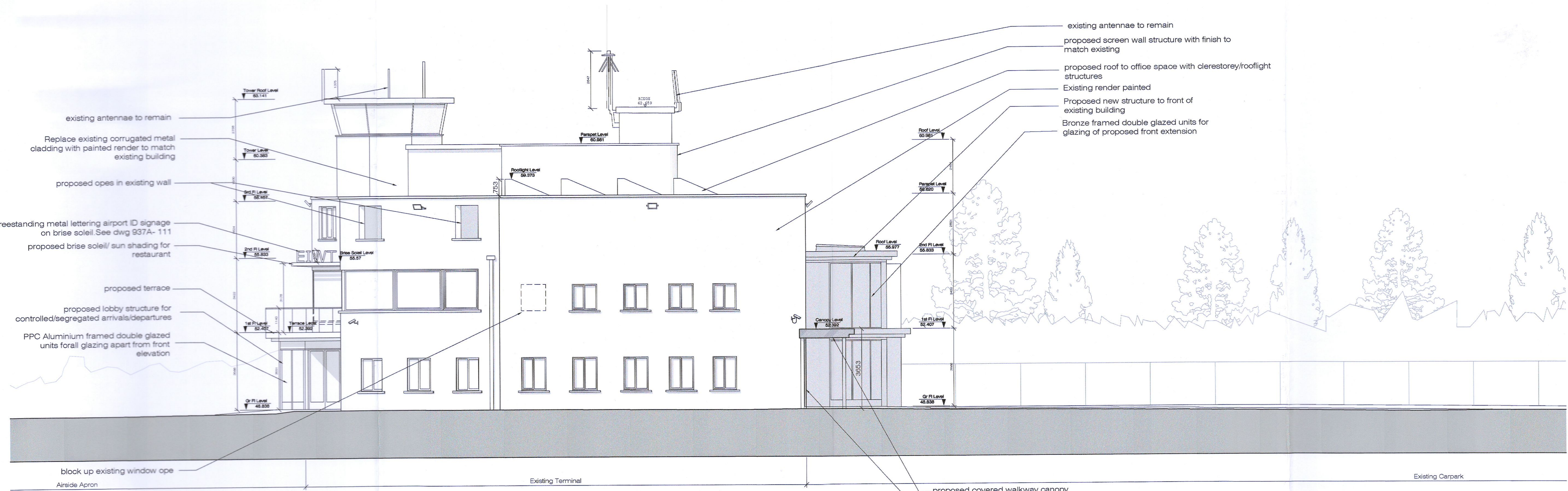
Proposed Northeast Elev 1:100
