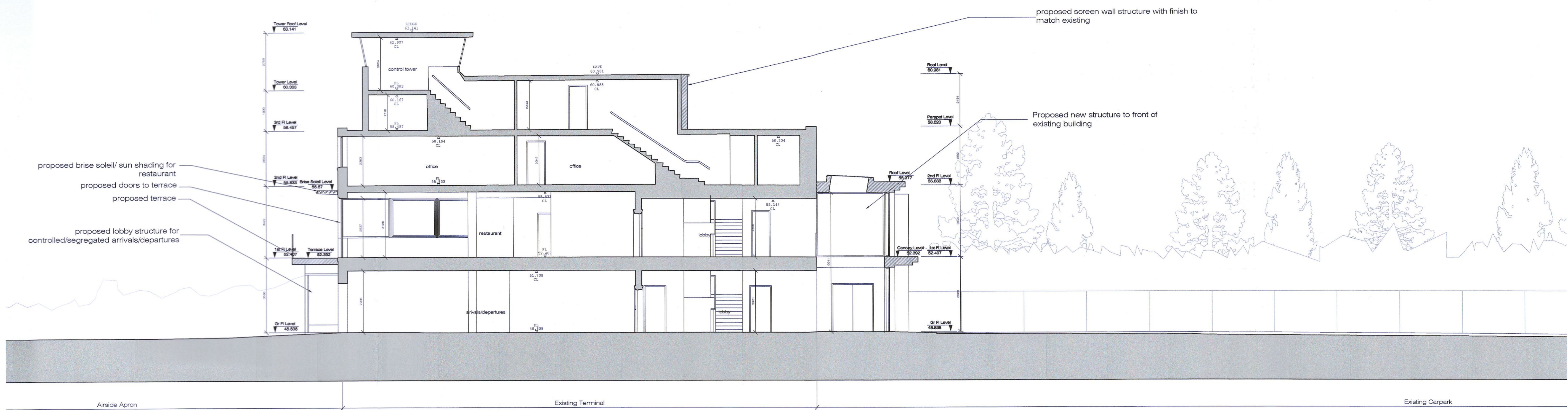
Proposed Section AA 1:100
