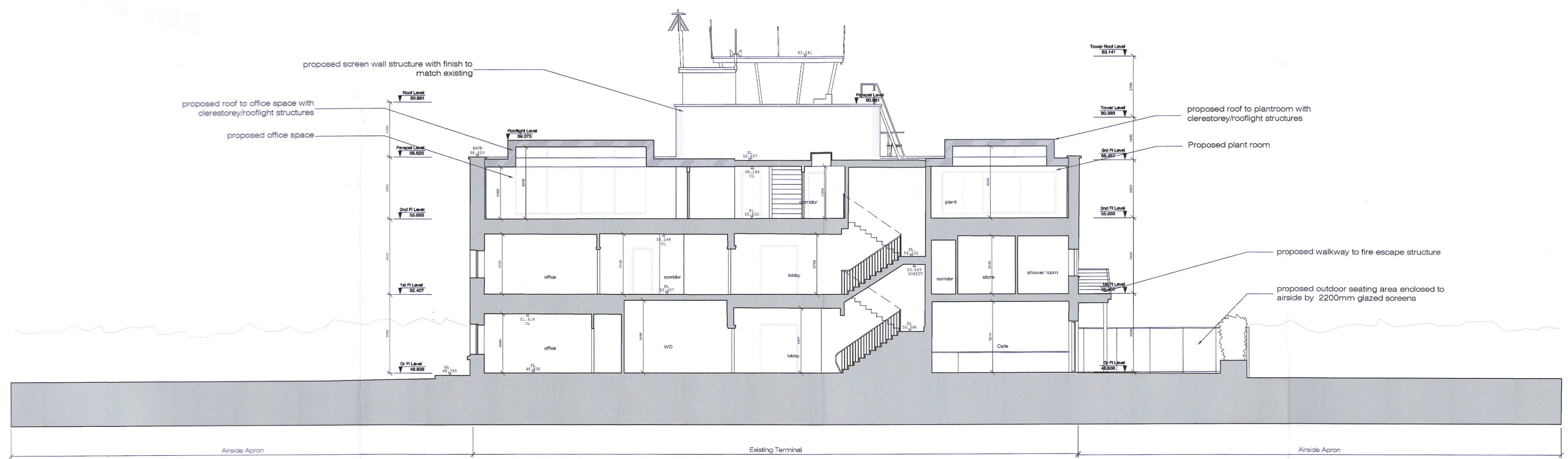
Proposed Section BB 1:100
