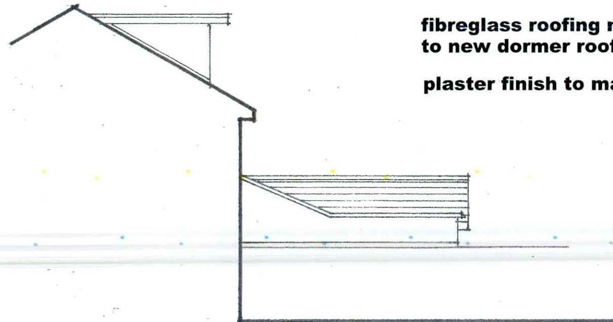
side elevation 1:100.
