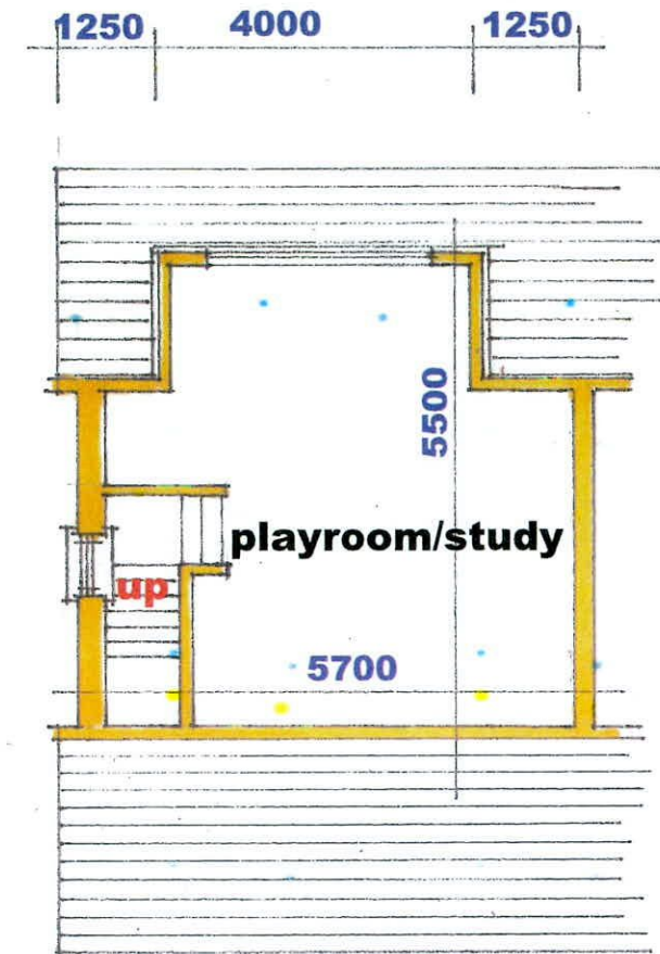
attic plan 1:100.
