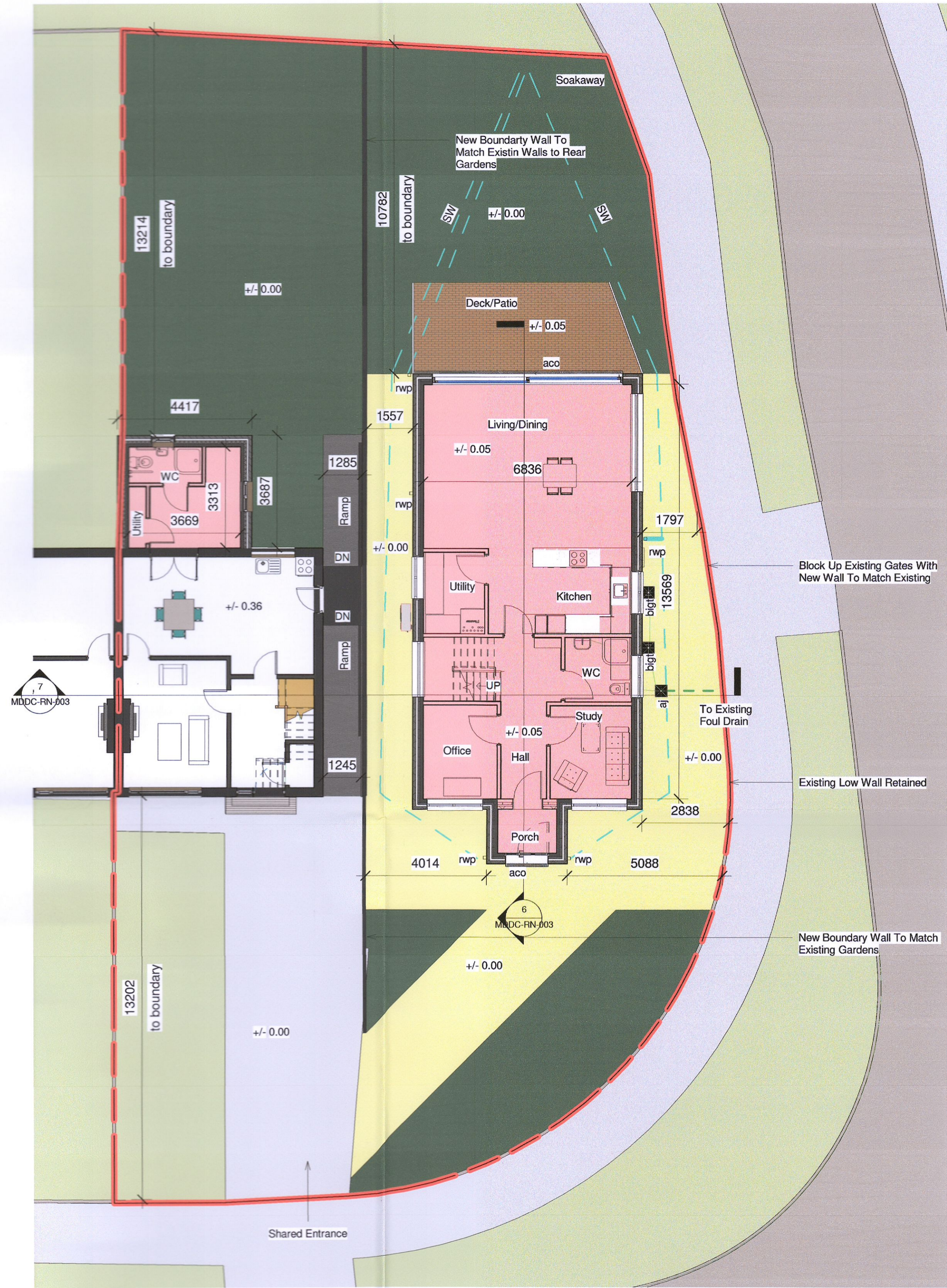
1 New Ground Floor 1 : 100
