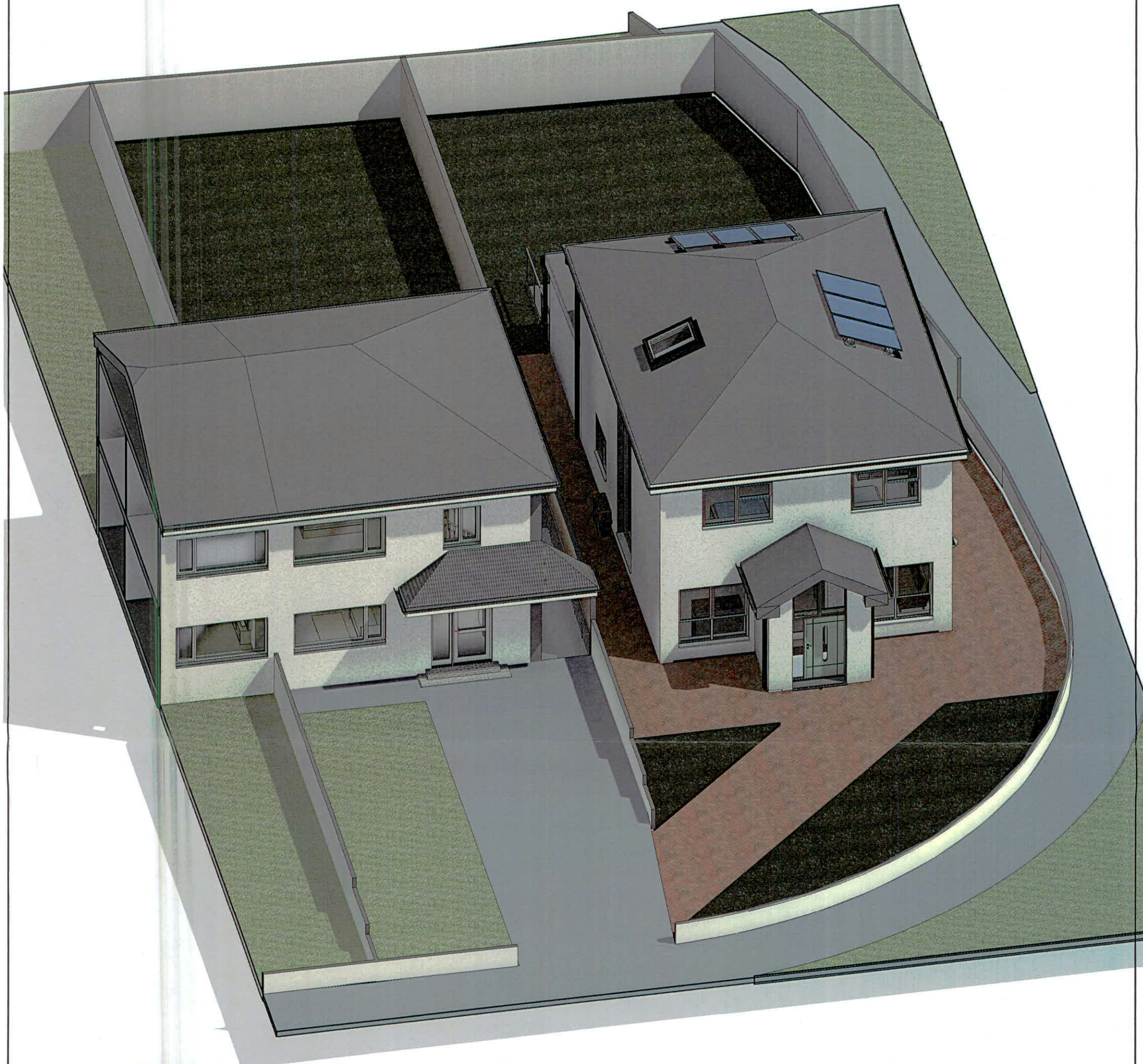
1 Proposed 3D front elevation
