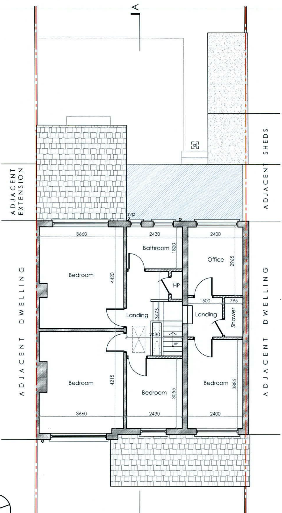
Existing First Floor Plan scale 1:100 @ A3
