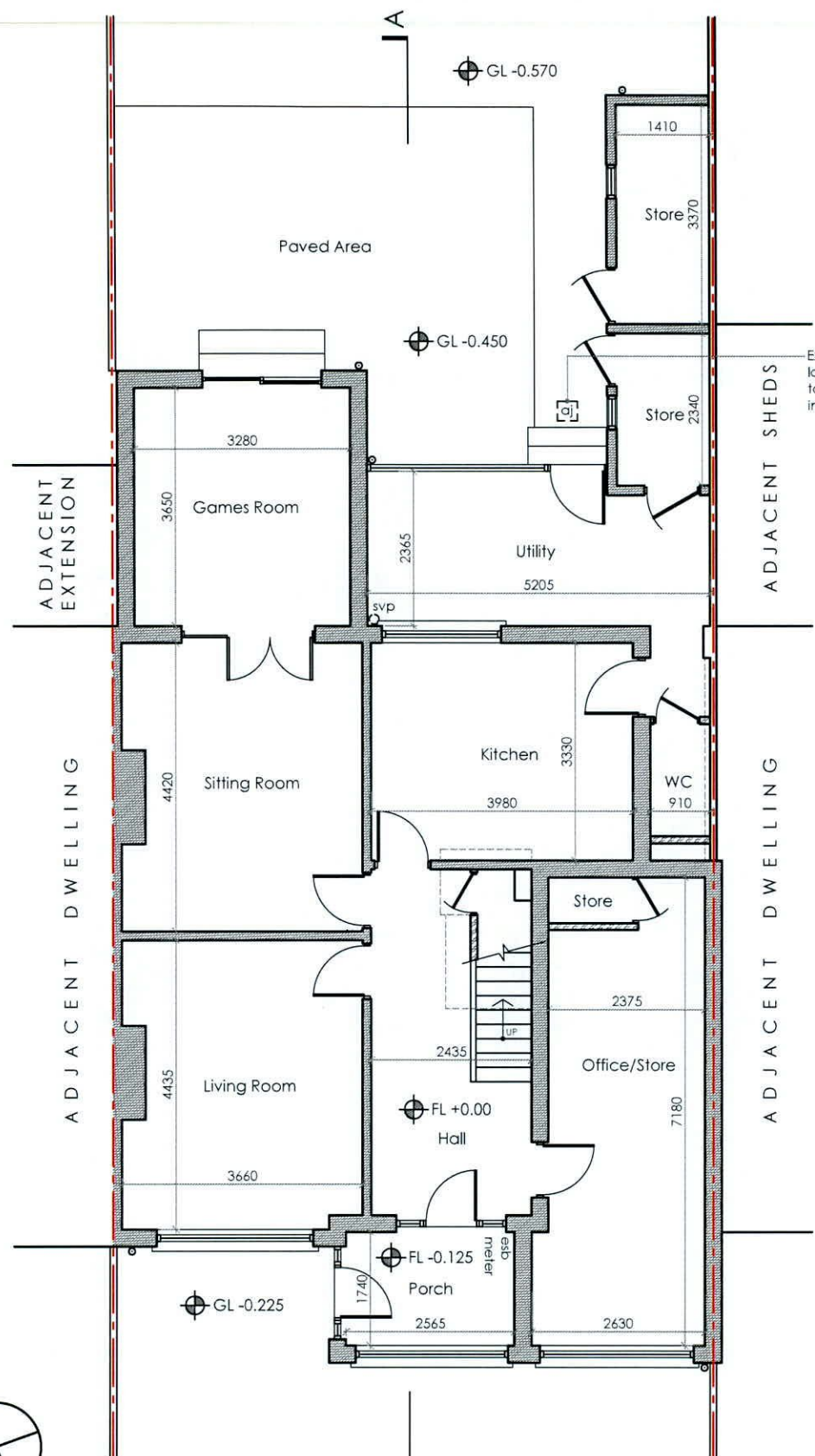
Existing Ground Floor Plan scale 1:100 @ A3
