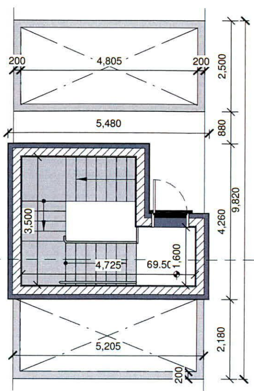
BB_00 - External Staircore _Ground Level 1 : 100
