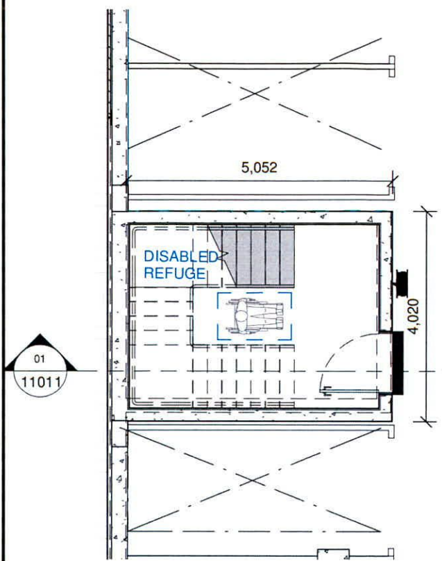
BB_B1 - Basement Level External Stairs 1 : 100
