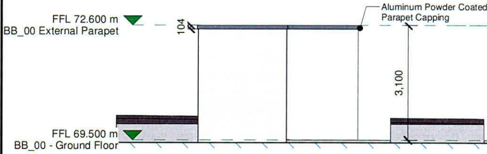
External Stairs_Front Elevation 1 : 100
