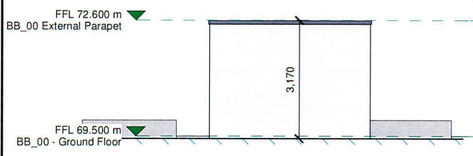
External Stairs_Rear Elevation 1 : 100
