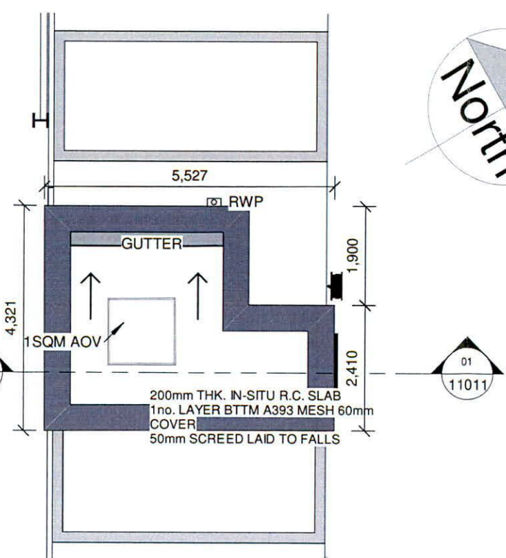
External Stairs Roof Plan 1 : 100
