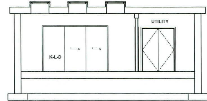
Section E-E 1:100
