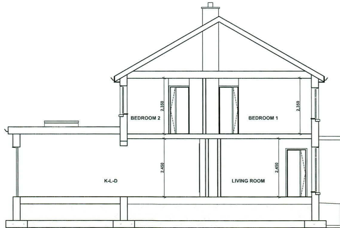
Section C-C 1:100
