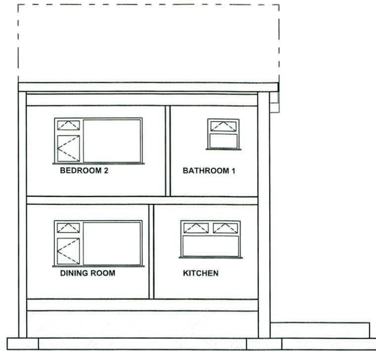
Section B-B 1:100
