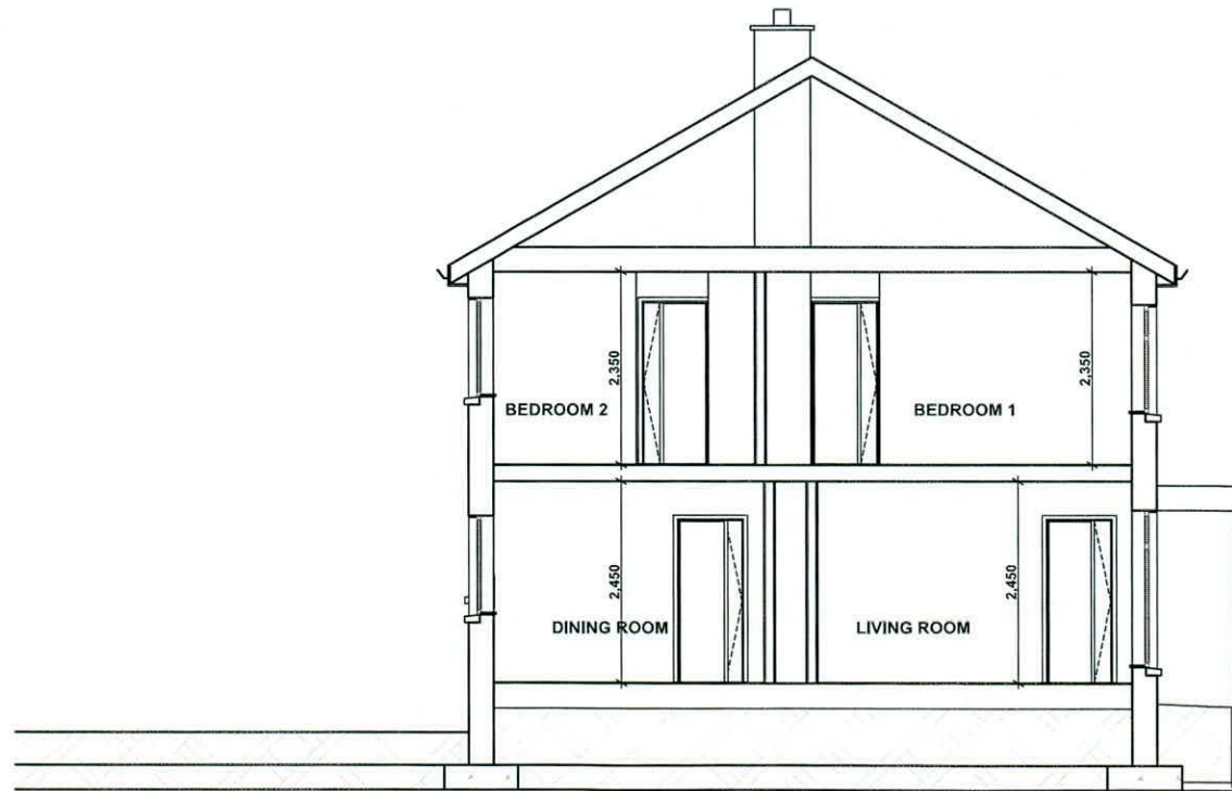
Section C-C 1:100
