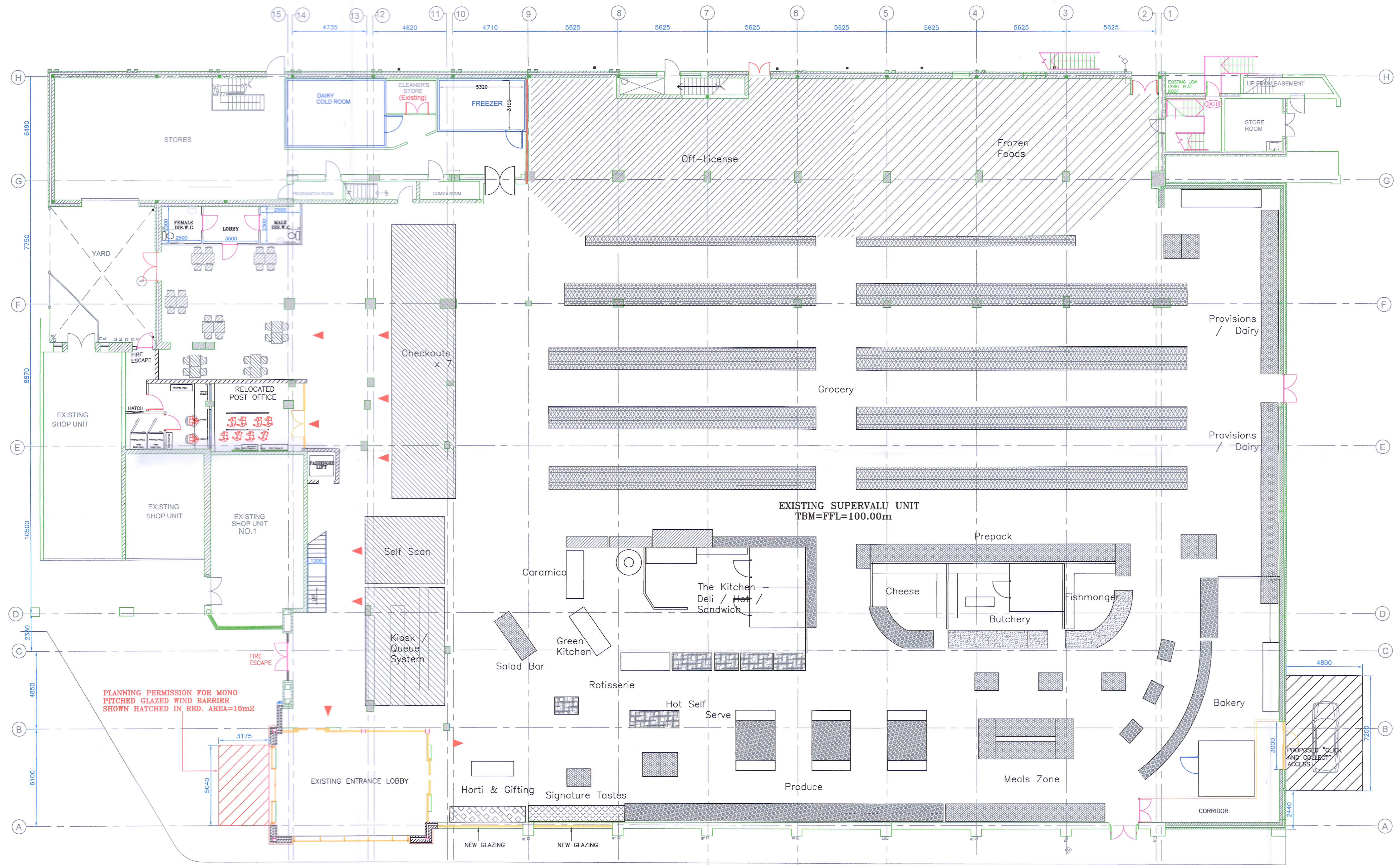
GROUND FLOOR PLAN SHOWING PROPOSED WIND BARRIER
