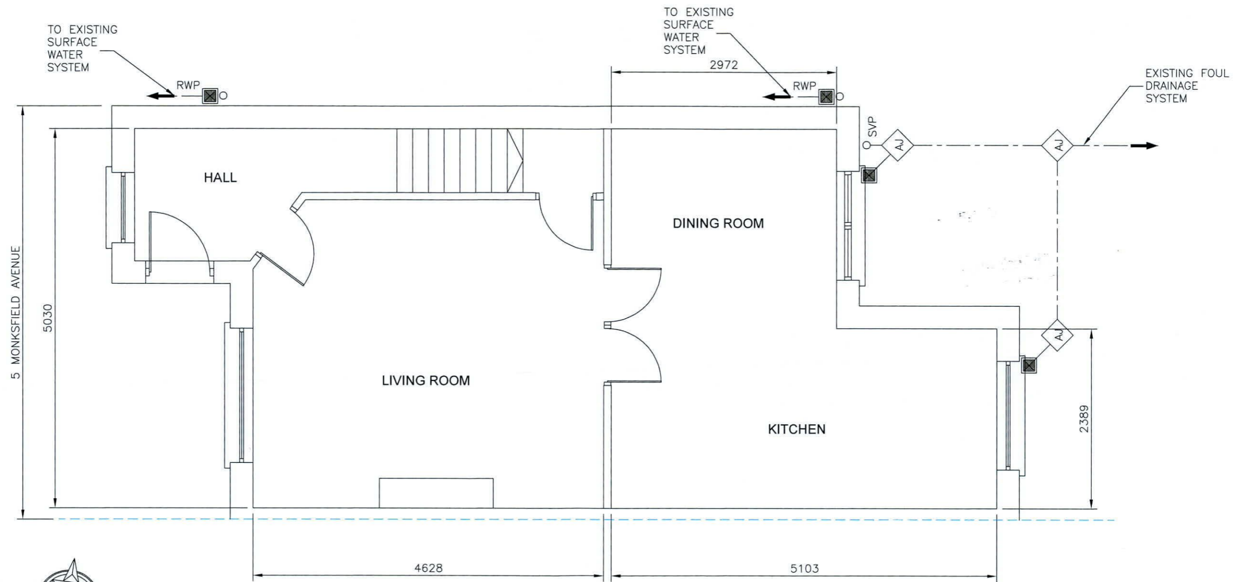
EXISTING GROUND FLOOR PLAN VIEW
