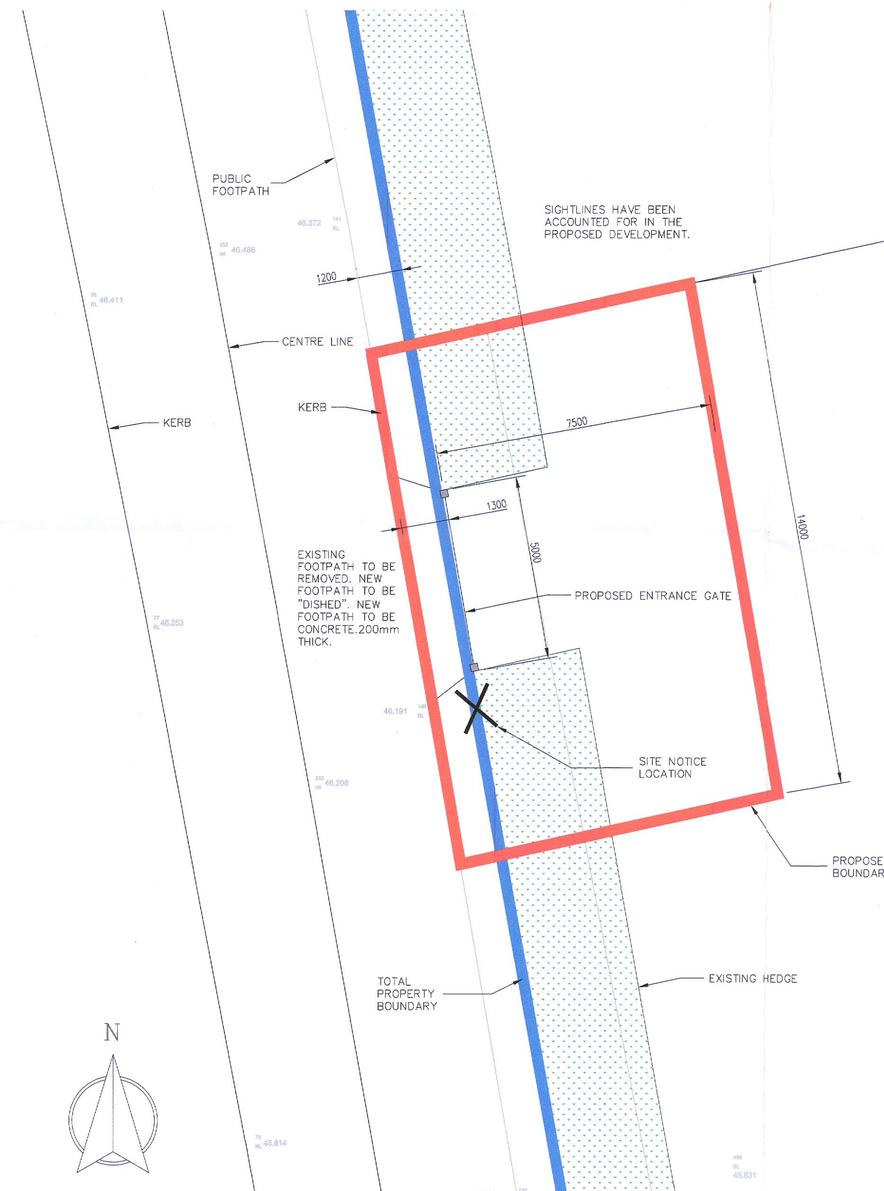
SIGHTLINES LOOKING SOUTH
