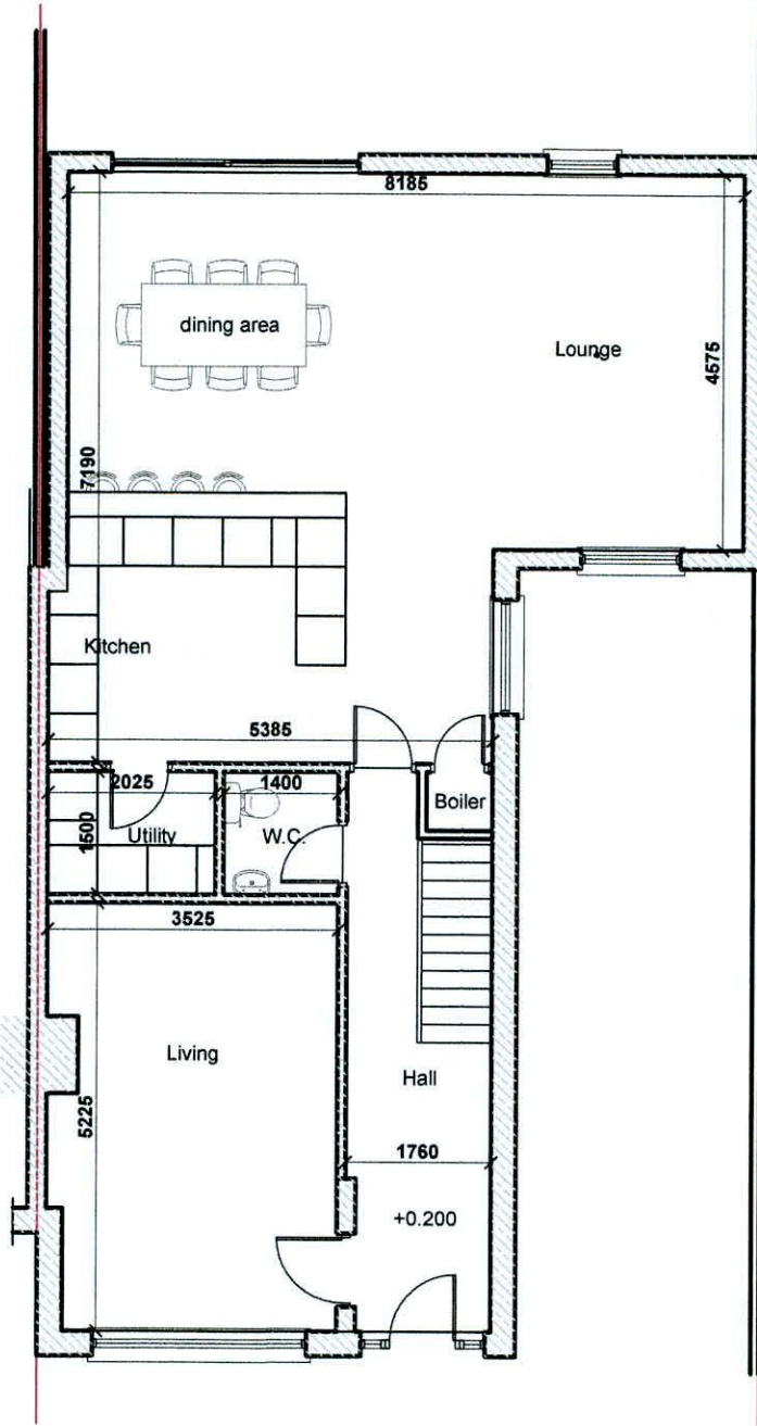
Proposed Ground Floor Plan Scale - 1:100 (No Change)
