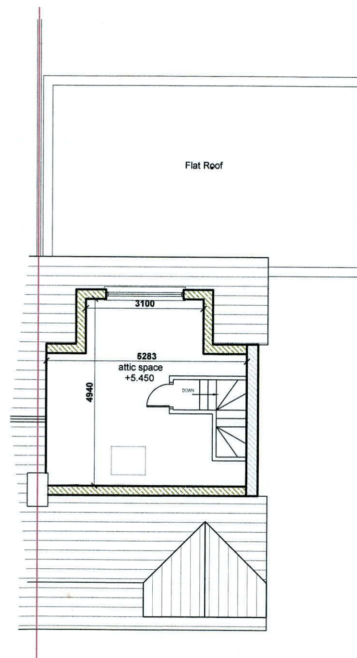
Proposed Attic Floor Plan Scale - 1:100
