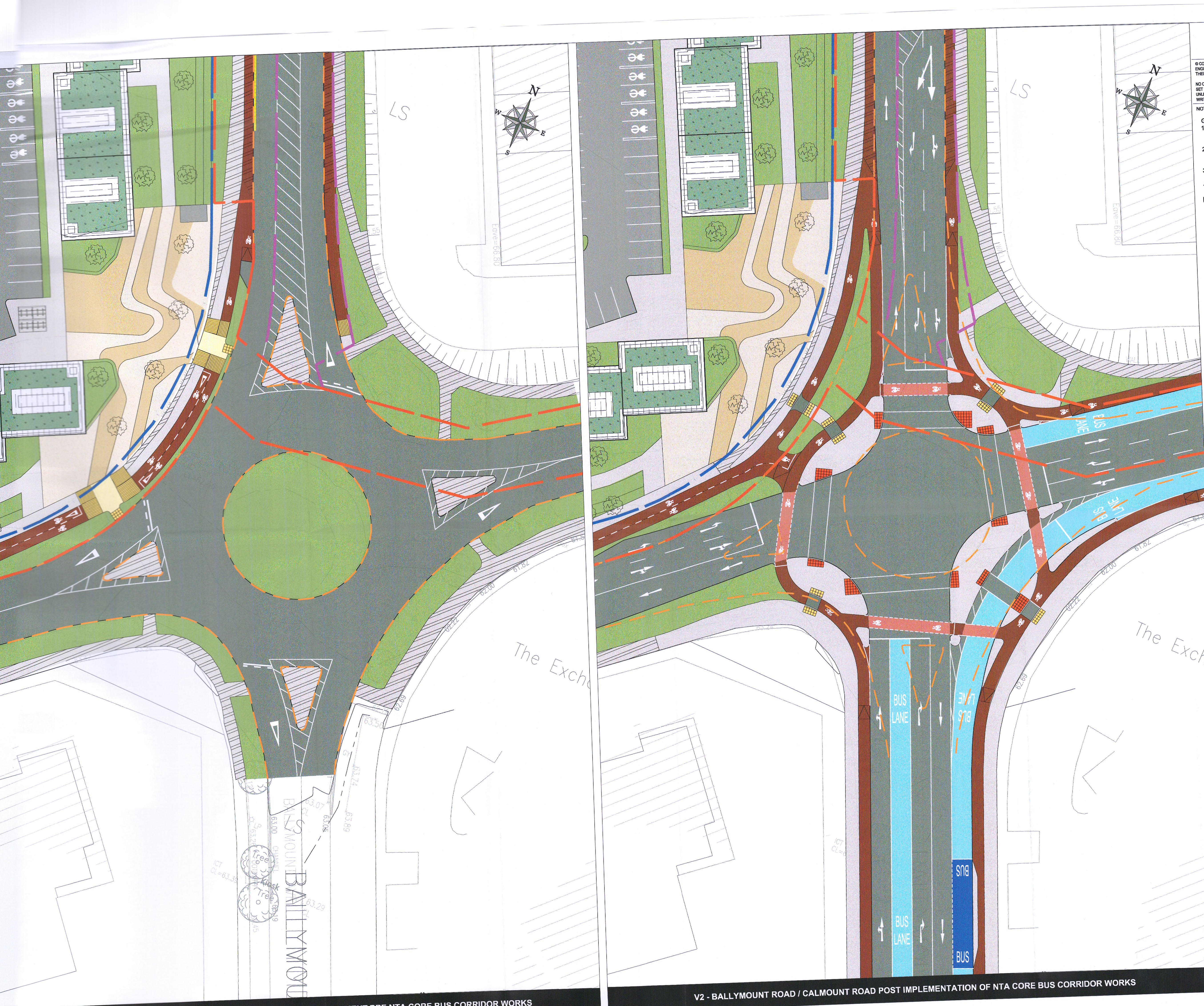
V1 - BALLYMOUNT ROAD / CALMOUNT ROAD PROPOSED ARRANGEMENT PRE NTA CORE BUS CORRIDOR WORKS
