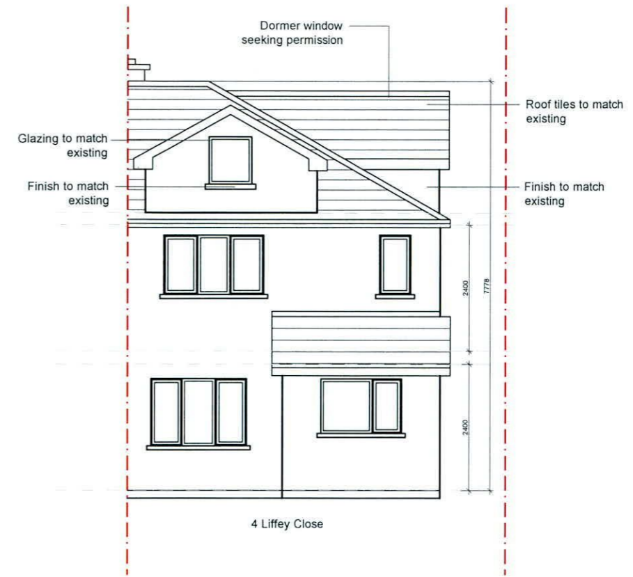
Rear (North-East) Elevation
