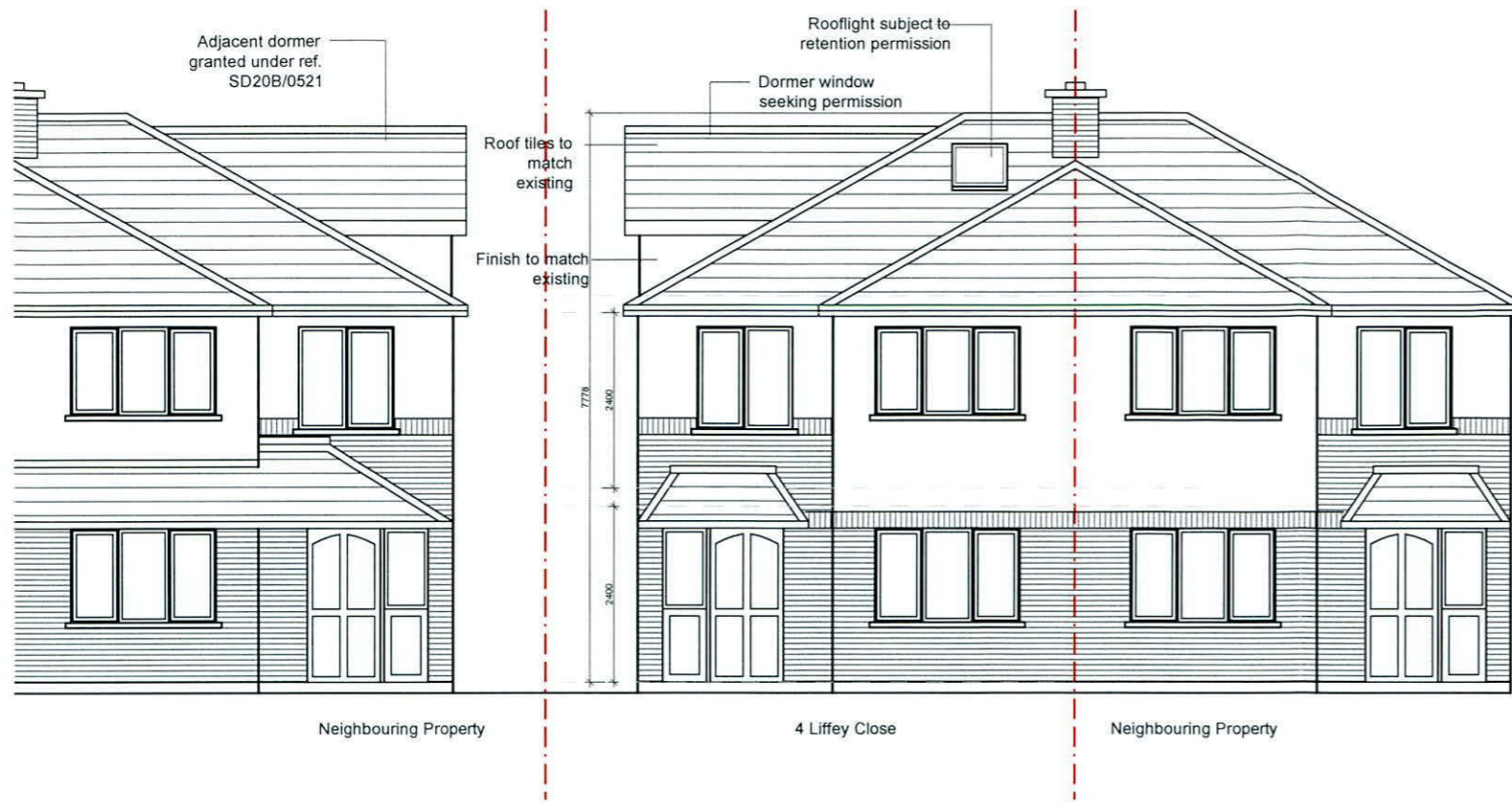
Front (South-West) Elevation / Context Elevation
