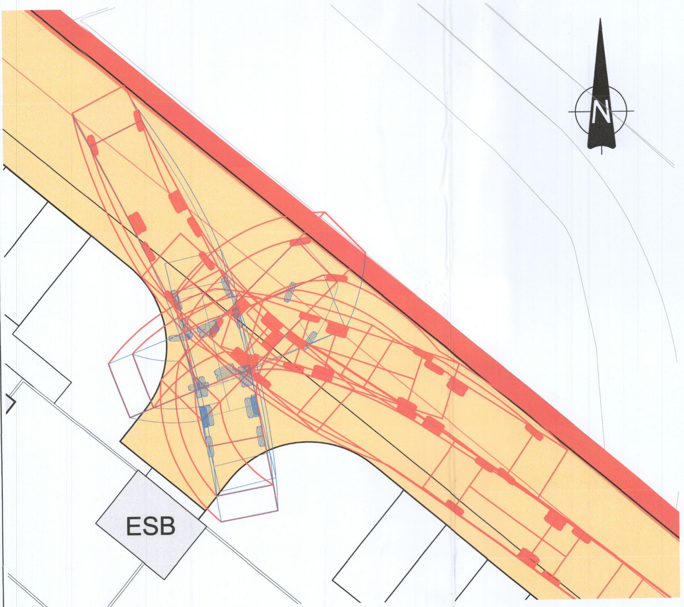
REFUSE ANALYSIS 7 SCALE 1:100
