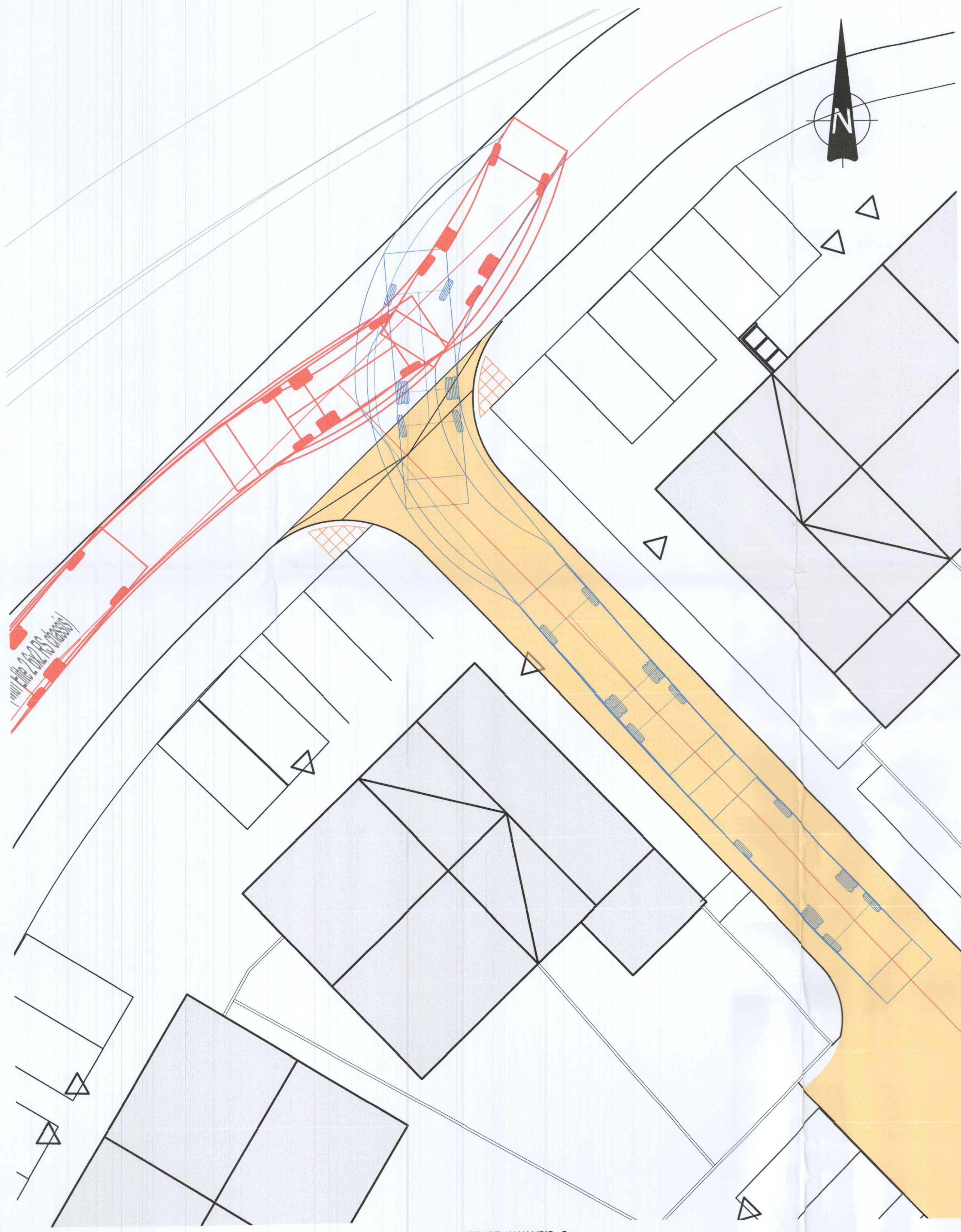
REFUSE ANALYSIS 8 SCALE 1:100
