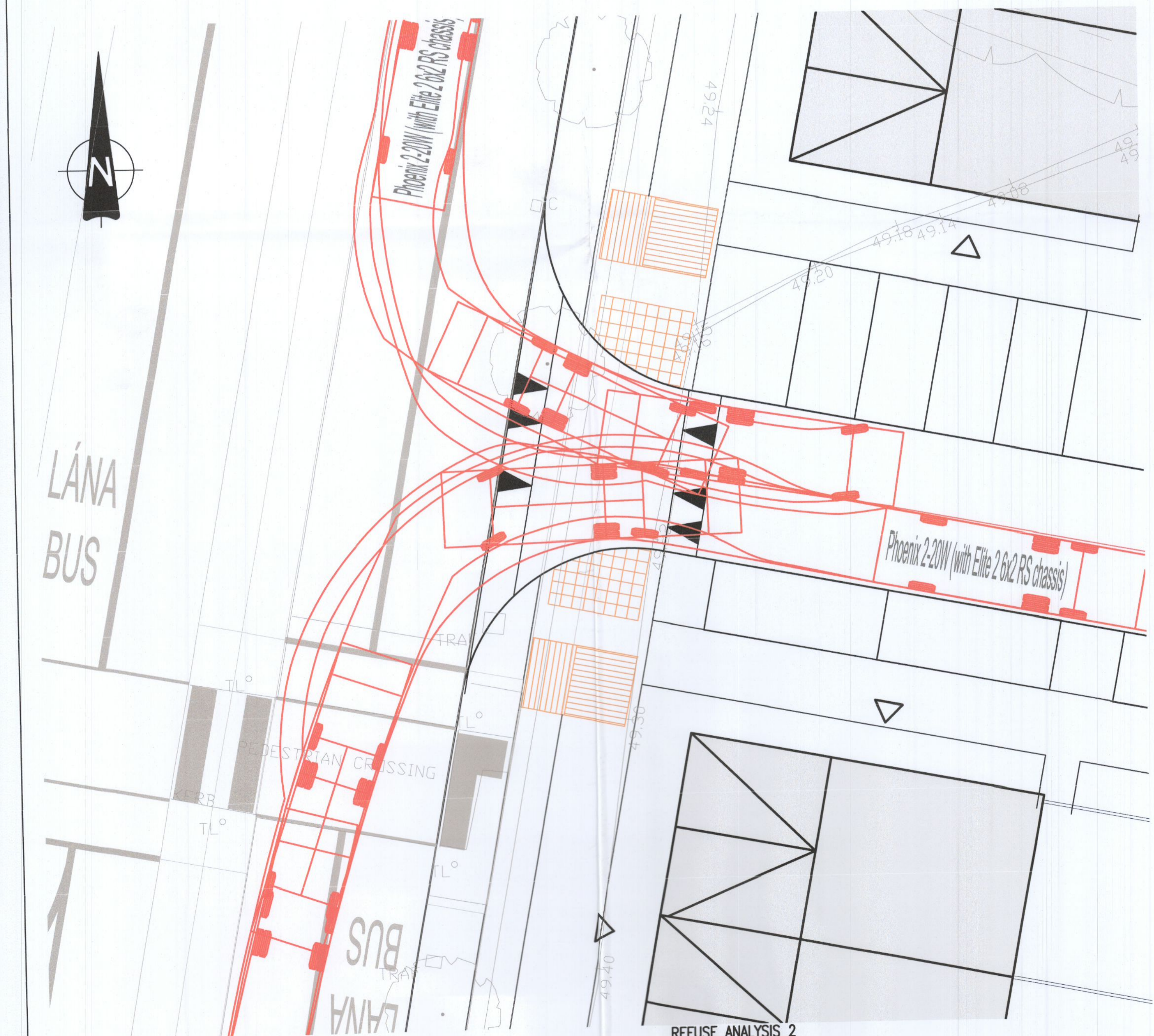
REFUSE ANALYSIS 2 SCALE 1:100
